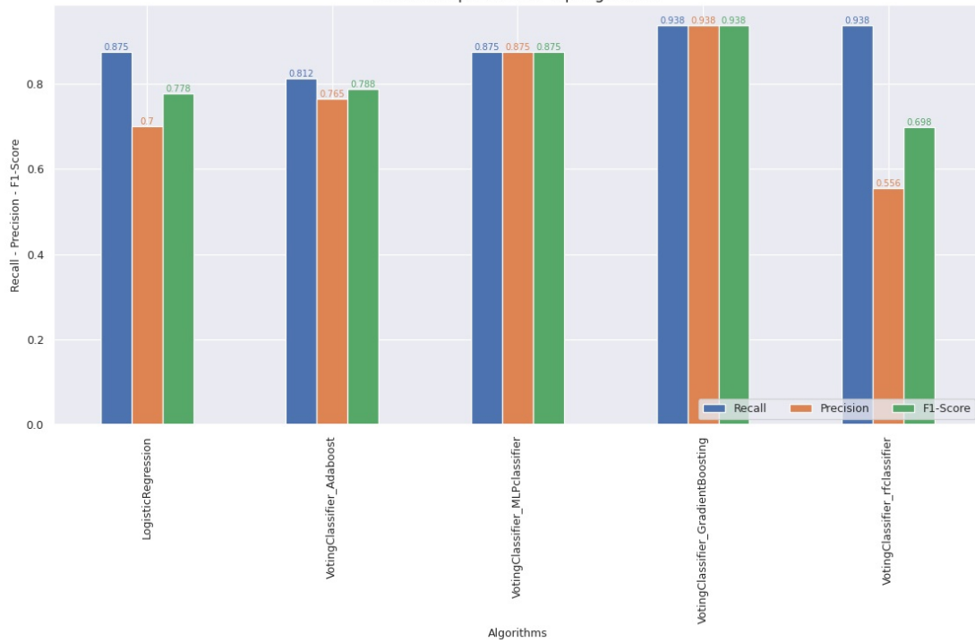
Visual Comparisons of Top Algorithms
