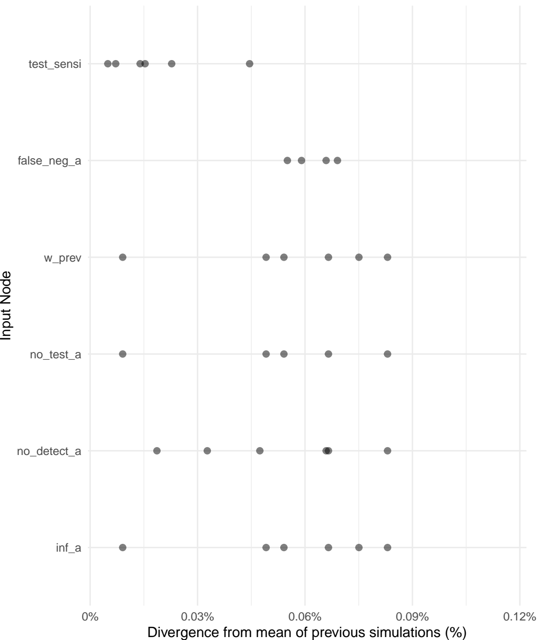
Divergence of the distribution in the last 10% simulations
