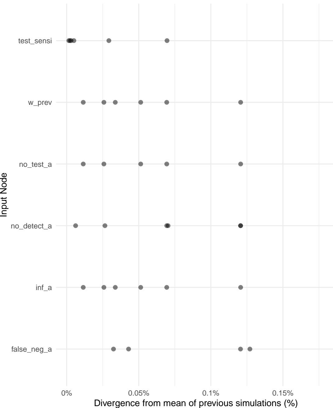
Divergence of the distribution in the last 5% simulations
