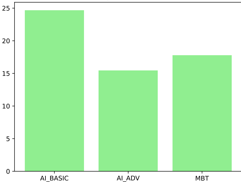
Average Test Suite Size
