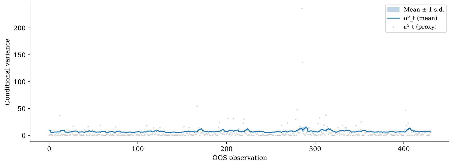
LSTM-SSE-t-Student — BTC-USD: Multi-seed \sigma^2_t stability
