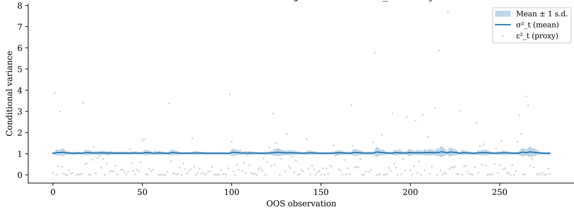
LSTM-SSE-t-Student — DJIA: Multi-seed \sigma^2_t stability
