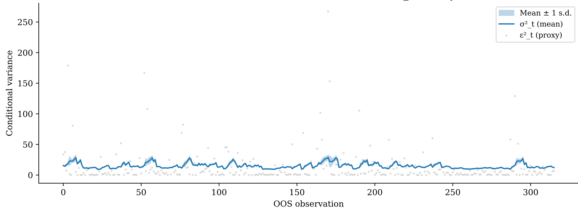
LSTM-SSE-t-Student — ETH-USD: Multi-seed \sigma^2_t stability
