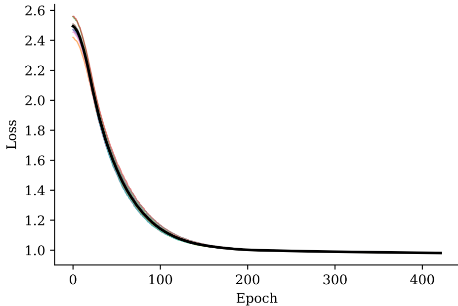
Train loss
