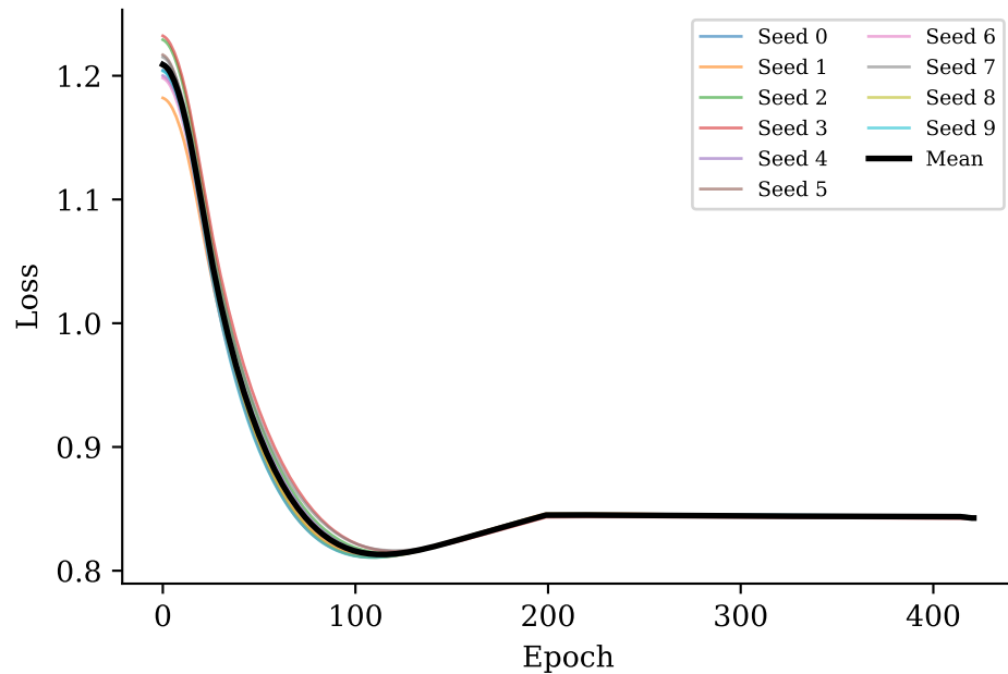
Validation loss
