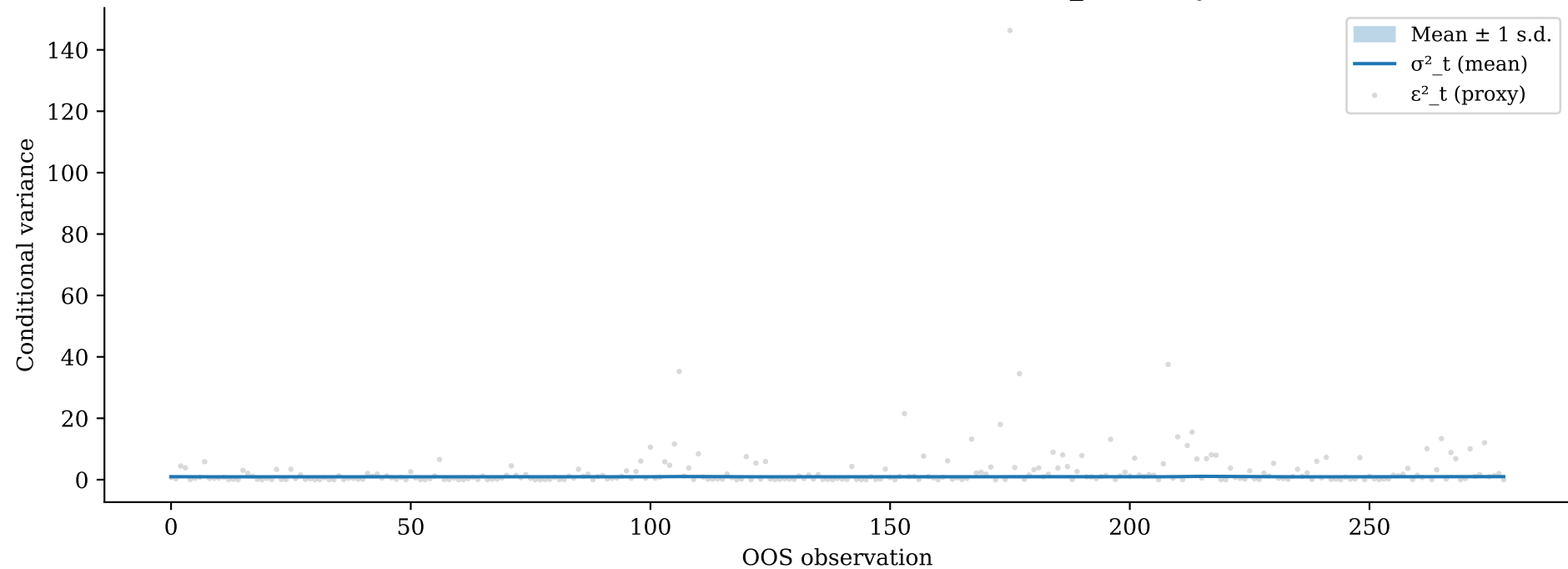
LSTM-SSE-t-Student — GOLD: Multi-seed \sigma^2_t stability
