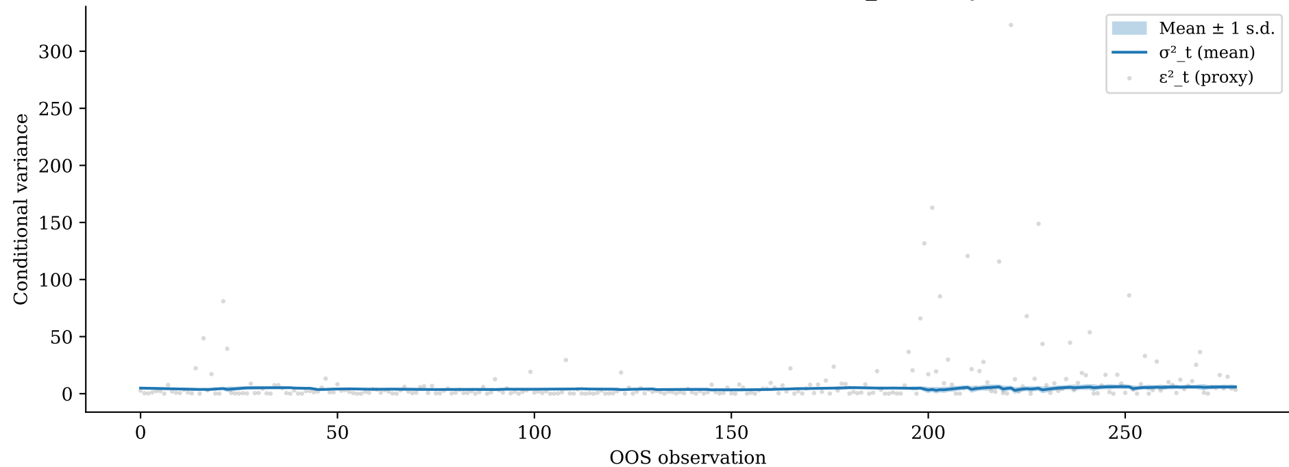
LSTM-SSE-t-Student — OIL: Multi-seed \sigma^2_t stability
