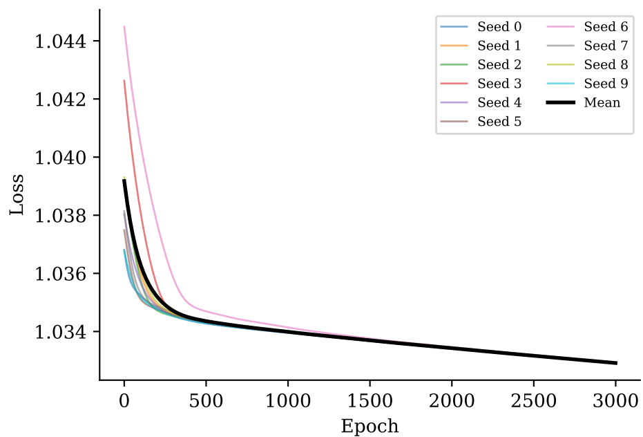
Validation loss
