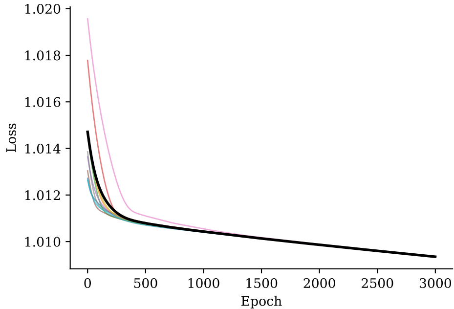
Train loss
