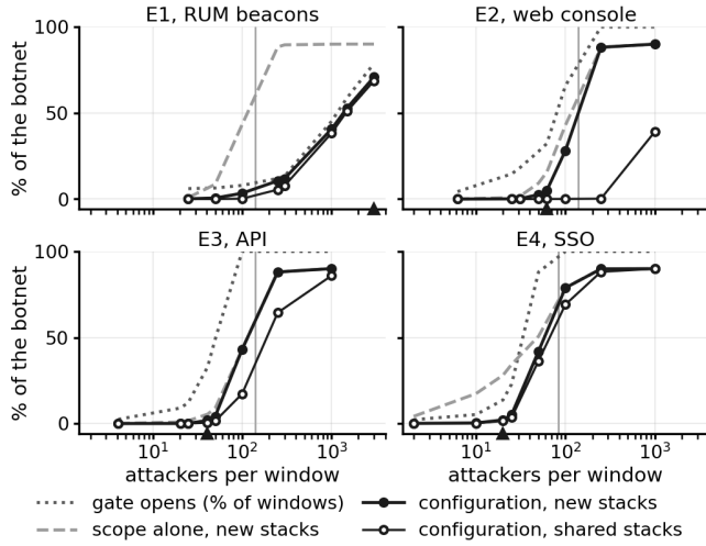
Fig. 2. What the binomial configuration stops, by the size of a 25-stack botnet, test days. Gate: windows where the distinct-origin gate opens. Scope alone: attackers the scope would block without the gate. Vertical line: floor on new stacks (Table V). Triangle: median window.
