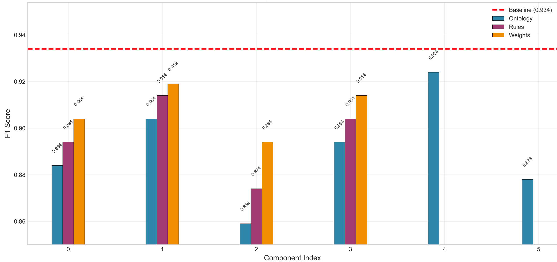
Ablation Study: Performance Comparison
