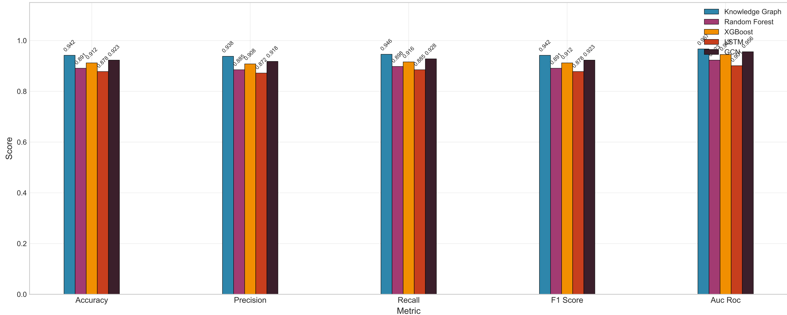
Classifier Performance Comparison
