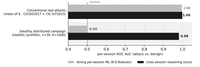
Fig. 4. Where cross-session reasoning is needed . On conventional real attacks a strong per-session classifier already saturates; only in the stealthy distributed regime does per-session detection collapse to chance while cross-session reasoning holds.
