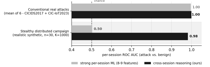
Fig. 4. Where cross-session reasoning is needed . On conventional real attacks a strong per-session classifier already saturates; only in the stealthy distributed regime does per-session detection collapse to chance while cross-session reasoning holds.
