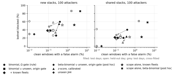
Fig. 4. Operating points on production traffic, 100 attackers per window (zero rates at 0.01%). Post hoc: the beta-binomial and the cross-fitted runs (grey).
