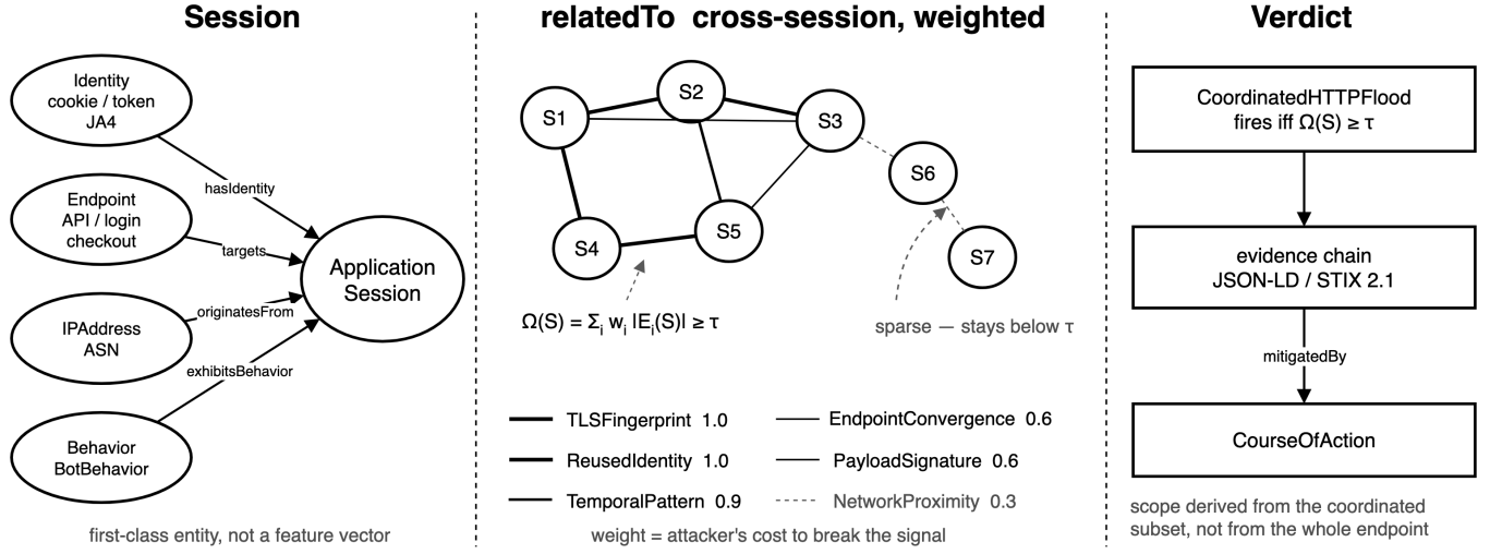
Fig. 1. Session-centric ontology. ApplicationSession is a first-class entity with typed primary relations to identity, origin, endpoint and behaviour; the weighted relatedTo family links sessions to each other; and the detection rule couples the symbolic verdict to a course of action whose scope is derived from the coordinated subset.
