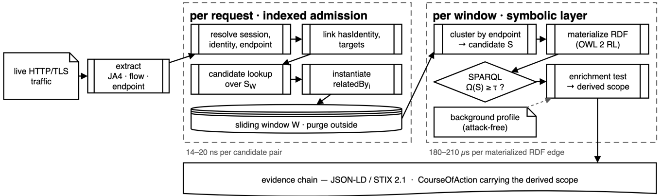
Fig. 2. Runtime pipeline. Admission runs per request over inverted indexes; RDF materialization and the \Omega aggregation run once per window. The enrichment test reads a background profile built outside attack episodes.
