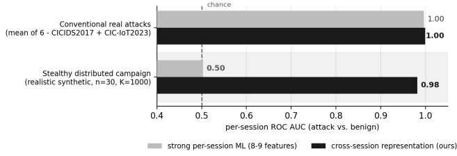
Fig. 4. Where cross-session evidence is needed . On conventional real attacks a strong per-session classifier already saturates; only in the stealthy distributed regime does per-session detection collapse to chance while cross-session representation remains discriminative.
