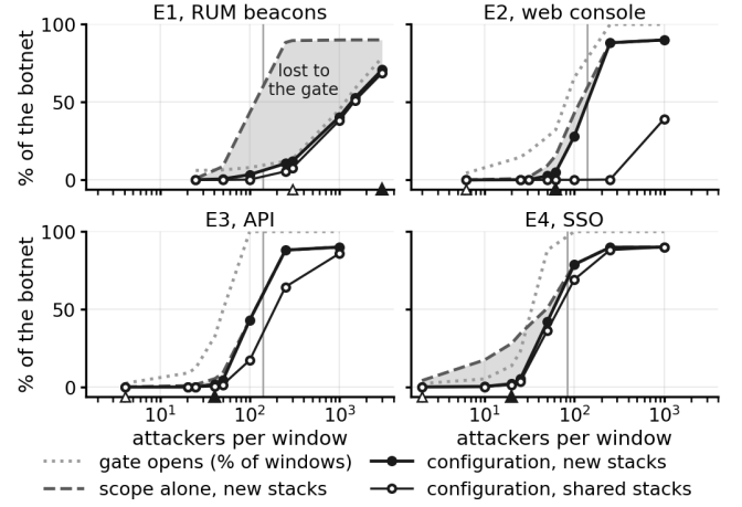
Fig. 2. What the binomial configuration stops, by the size of a 25-stack botnet, test days. Gate: windows where the distinct-origin gate opens. Shaded: attackers the scope alone would block but the gate lets through, most of a small botnet on the busiest endpoint. Vertical line: floor on new stacks (Table V). Triangles: the median window (filled) and a tenth of it (open).
