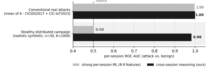
Fig. 3. Where cross-session reasoning is needed . On conventional real attacks a strong per-session classifier already saturates; only in the stealthy distributed regime does per-session detection collapse to chance while cross-session reasoning holds.
