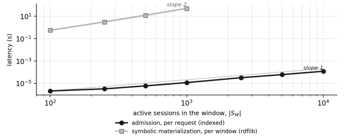
Fig. 4. Cost of the two layers against window occupancy. Per-request admission is linear in |S_W| and stays in the microsecond range; per-window symbolic materialization is linear in the number of RDF edges, which is itself quadratic in |S_W| . Reference slopes anchored on the first point of each series.
