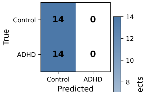
Majority-class Dummy
