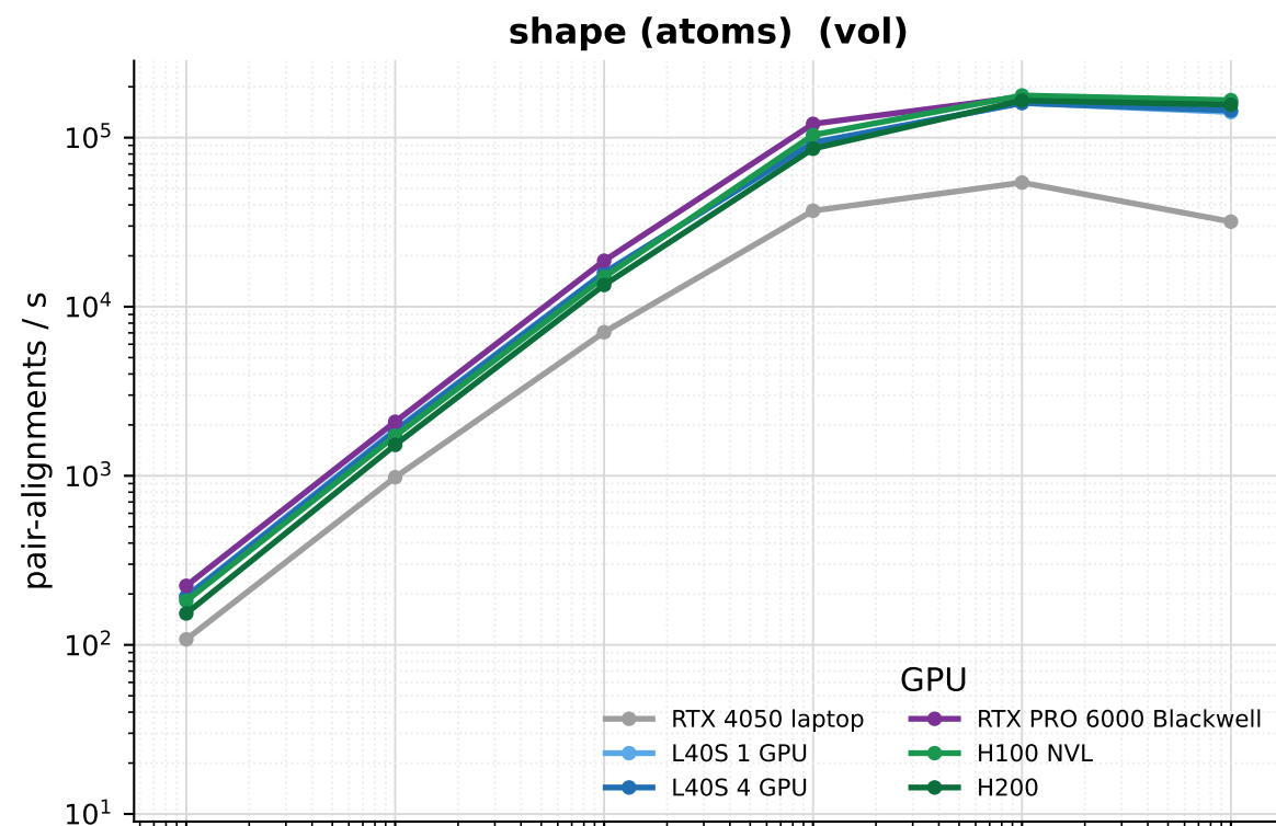
fast_shepherd_score throughput vs batch size, per mode and GPU (same-size bucket)
