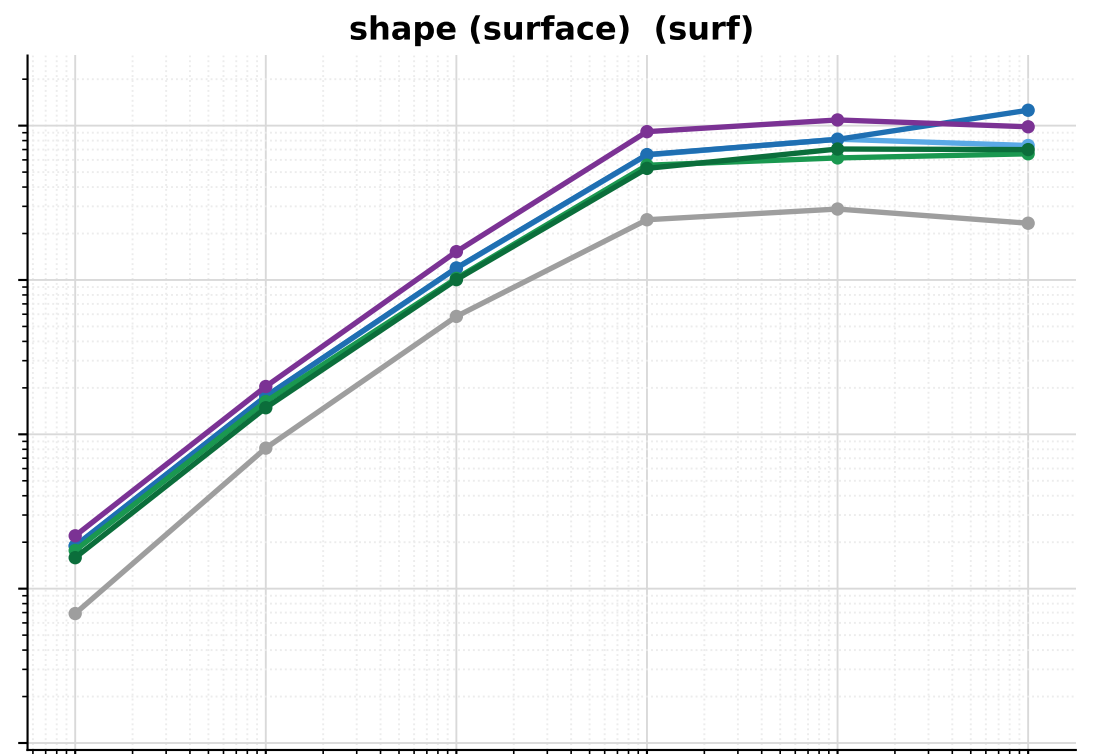
fast_shepherd_score throughput vs batch size, per mode and GPU (same-size bucket)
