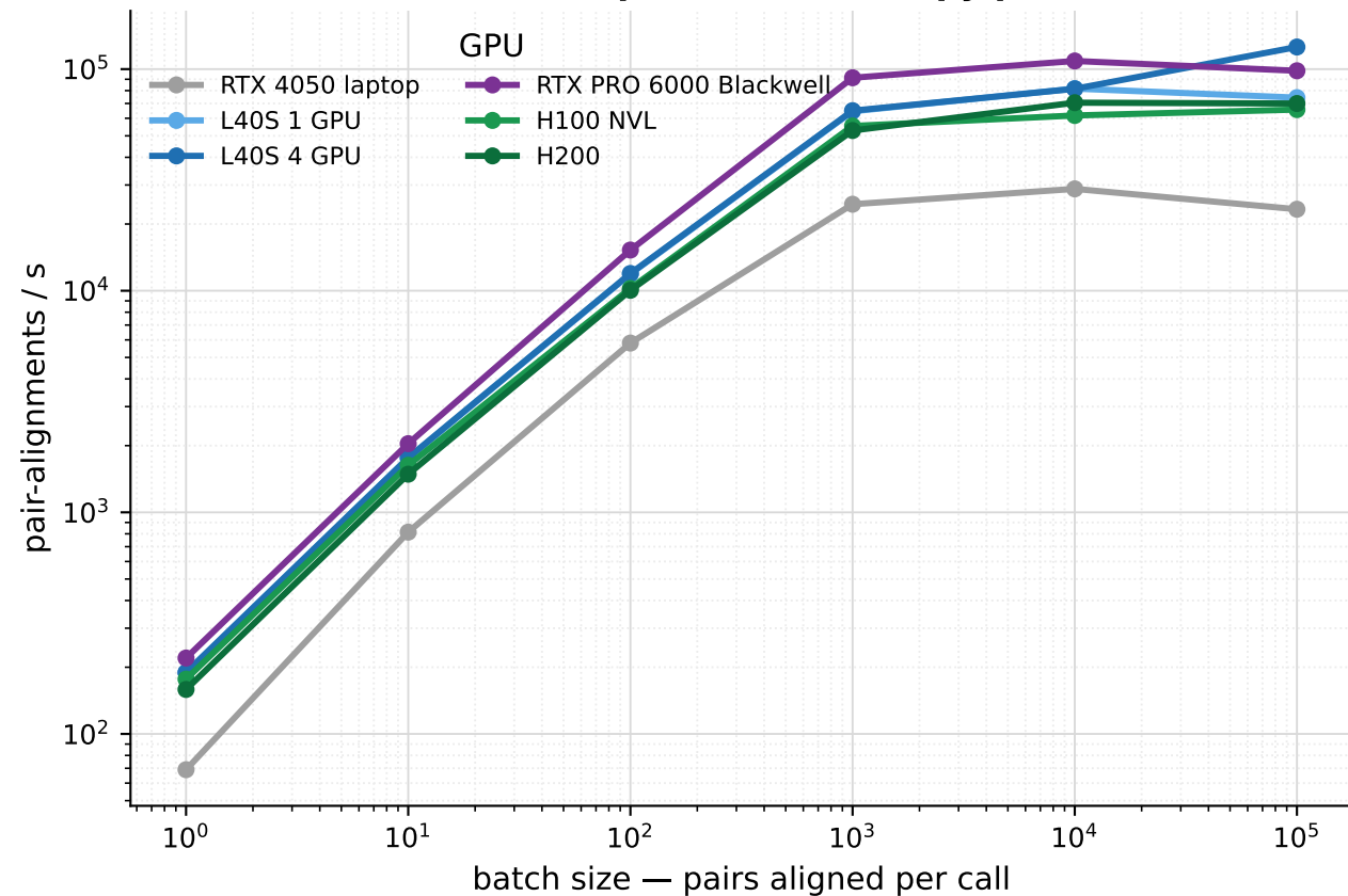
Throughput scales with batch size (surface-shape mode, self-copy pairs)
