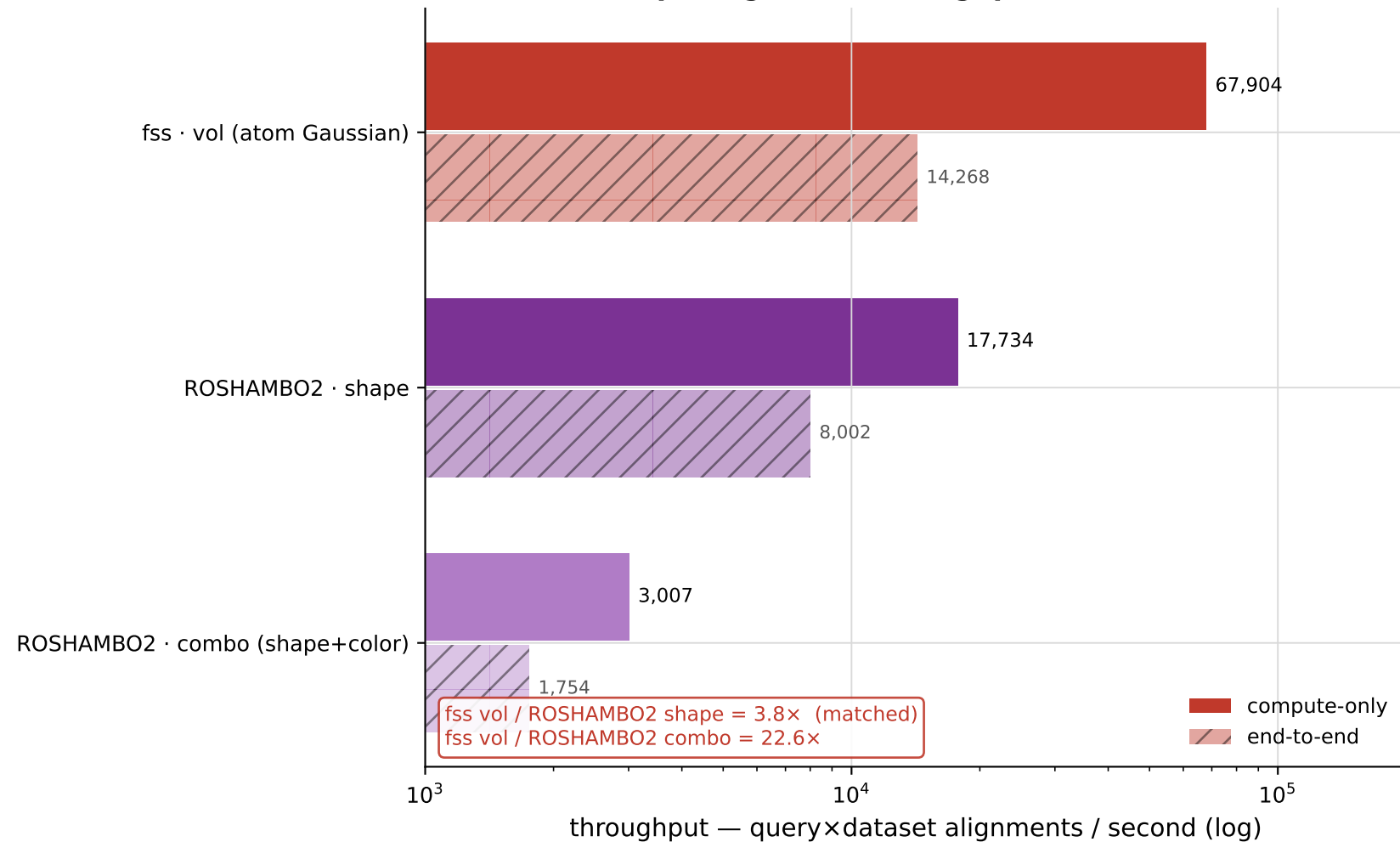
Shape-alignment throughput on one GPU
