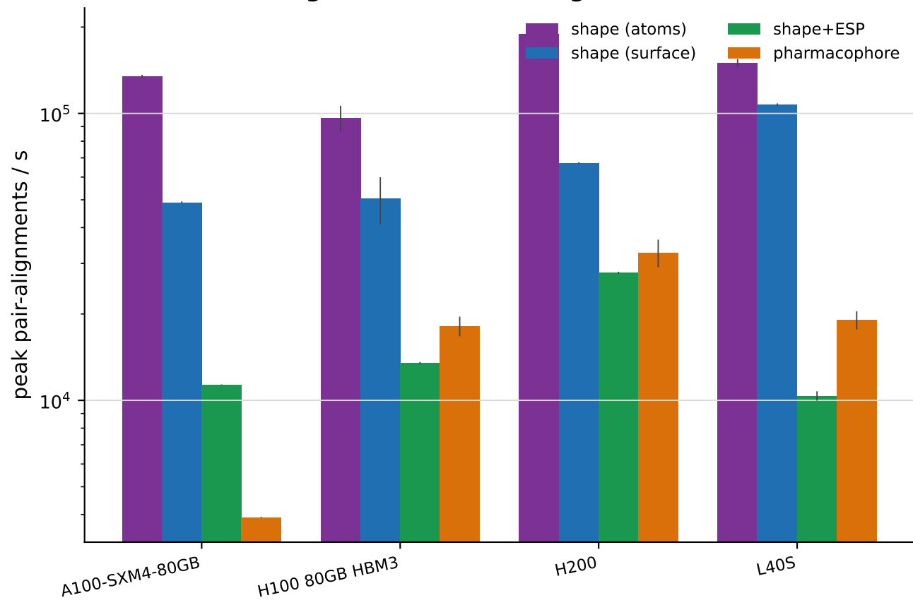
Peak throughput per mode (no clean generational ordering — see surf vs vol)
