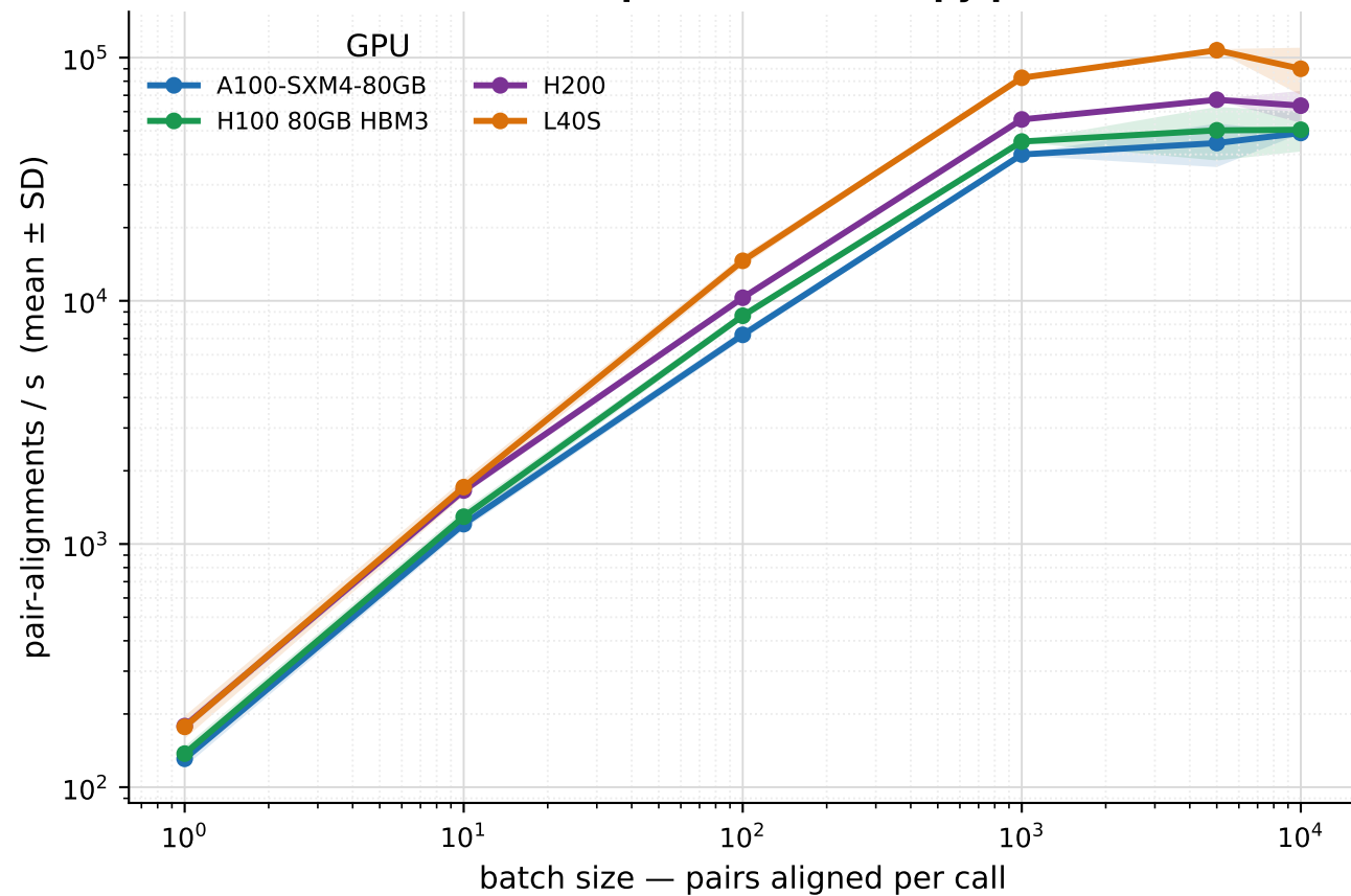
Throughput rises with batch size, then saturates (surface-shape mode, self-copy pairs)
