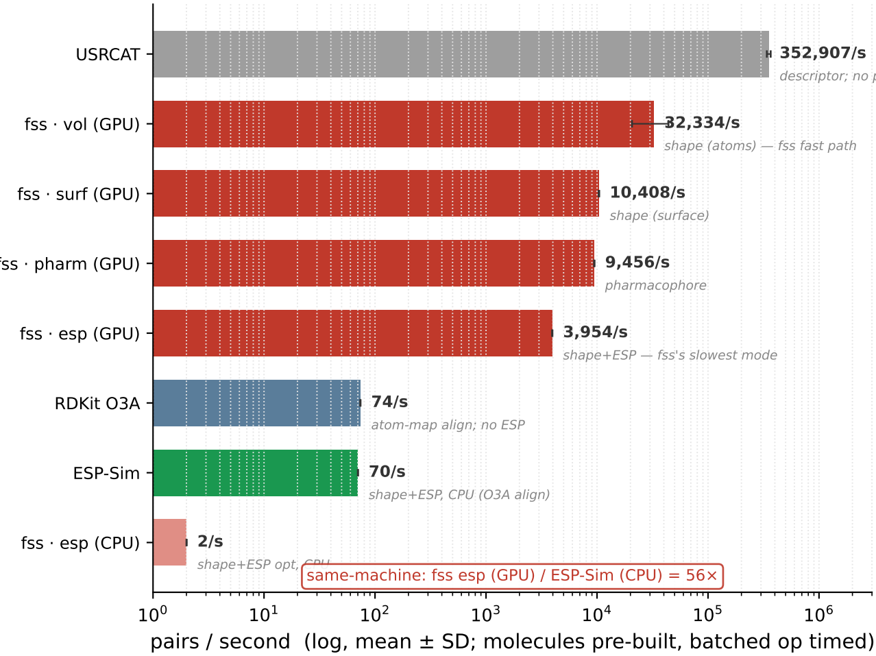
Throughput — same machine, every tool
