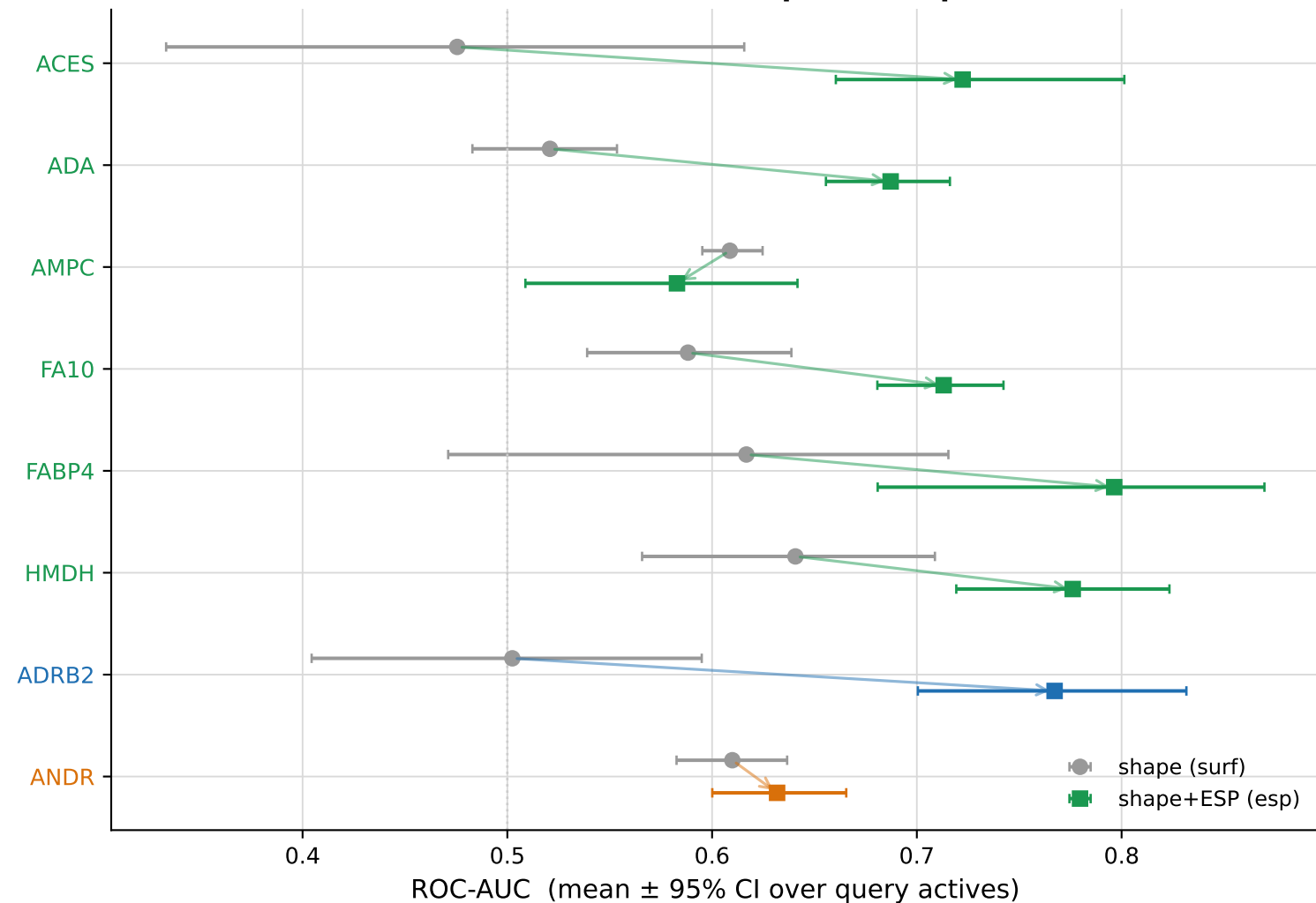
Retrieval at \lambda=0.003 : shape \rightarrow shape+ESP
