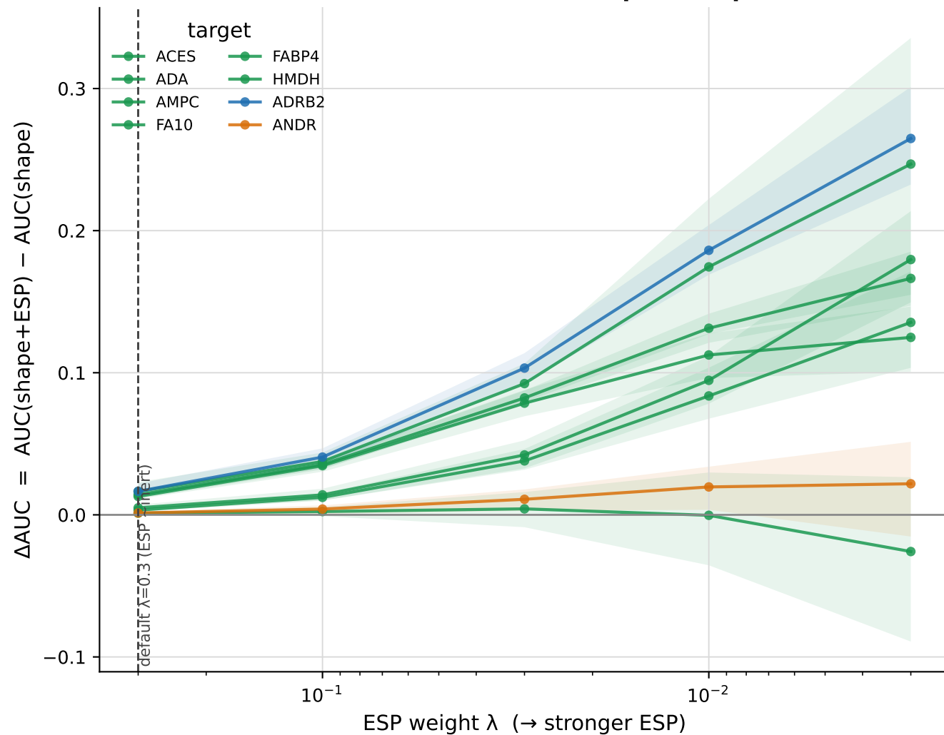
ESP ablation vs \lambda — benefit is pocket-specific
