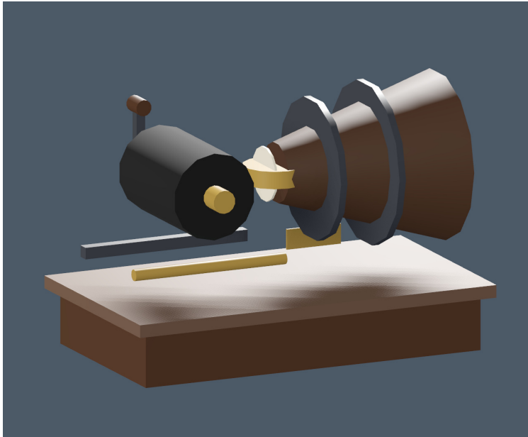
Drive and horn | current model / neutral light
