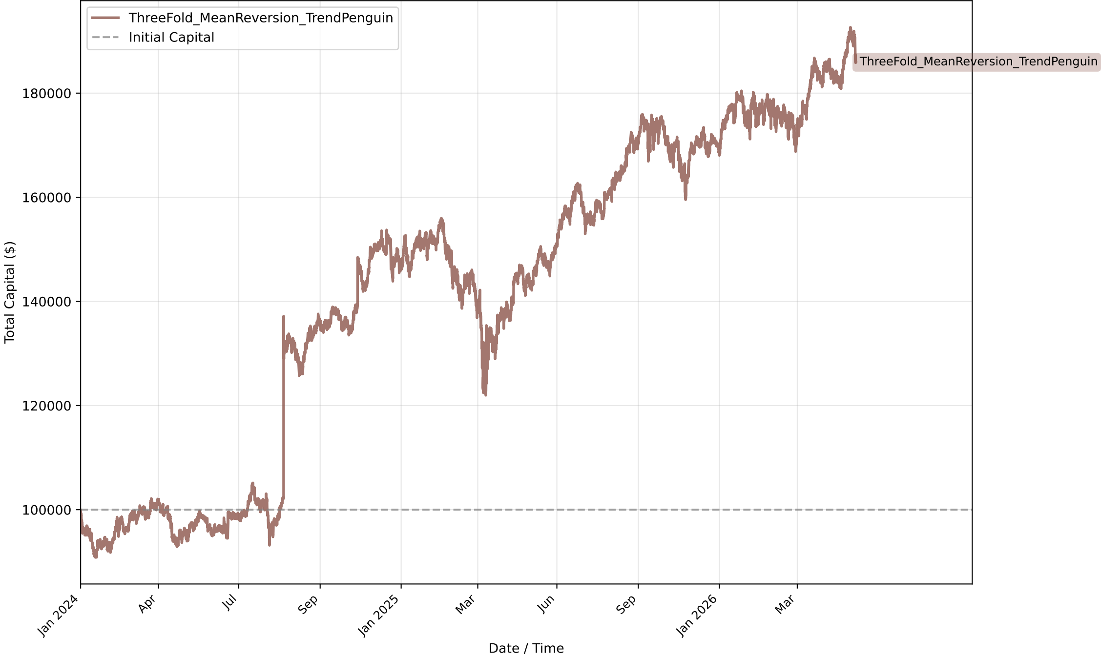
Capital Curve: ThreeFold_MeanReversion_TrendPenguin (LIST_5)
