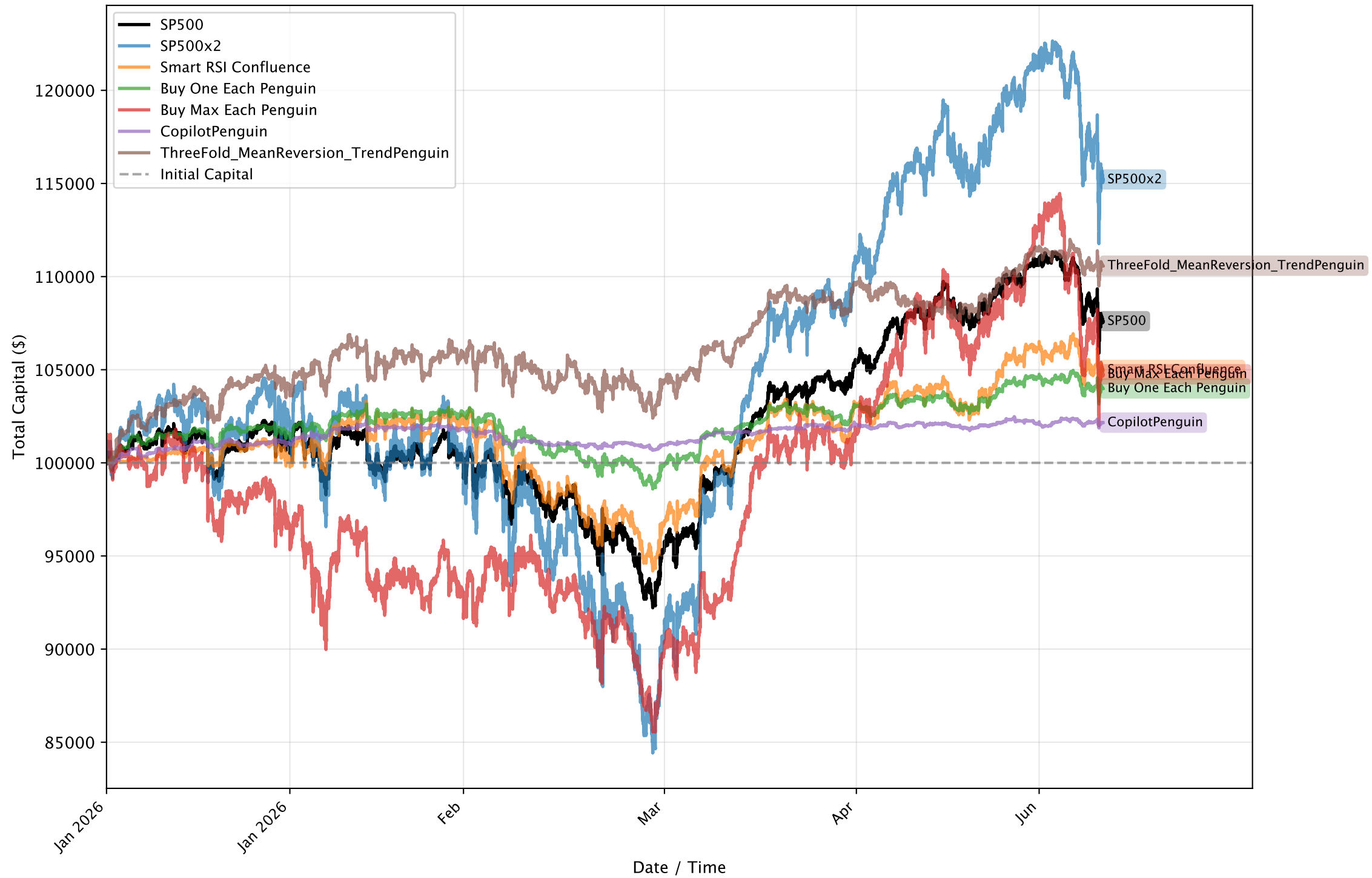
Penguin Capital Curves (LIST_3) (26-01-01 to 26-06-09)
