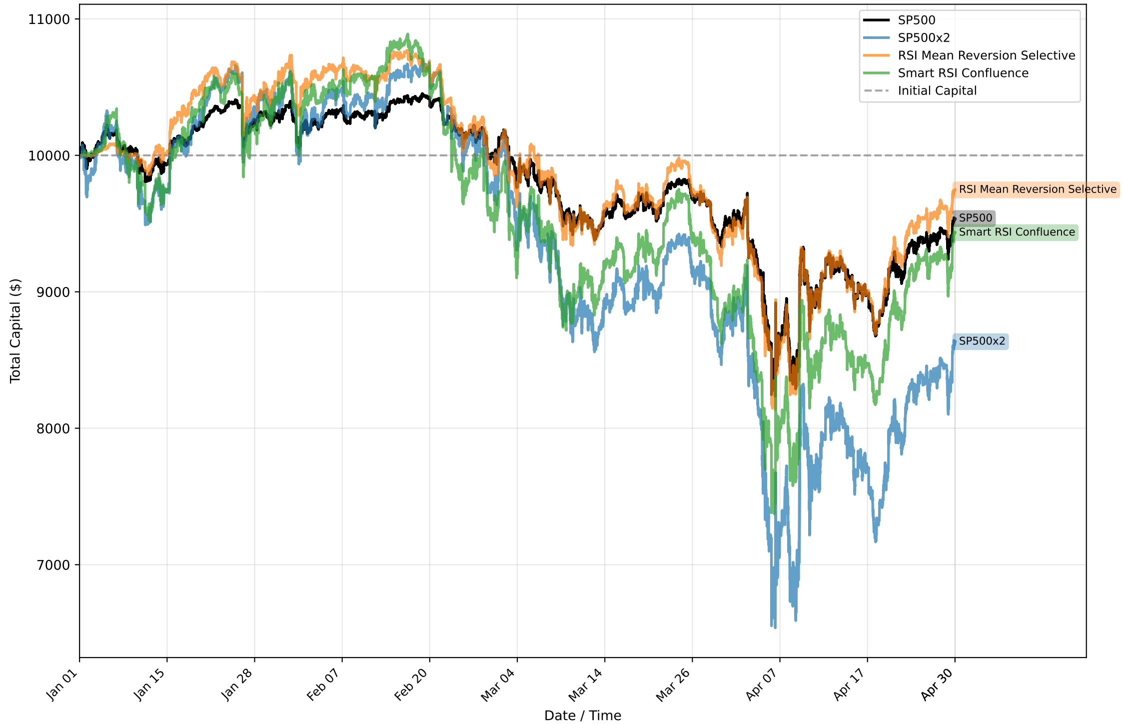
Penguin Capital Curves (25-01-01 to 25-04-30)
