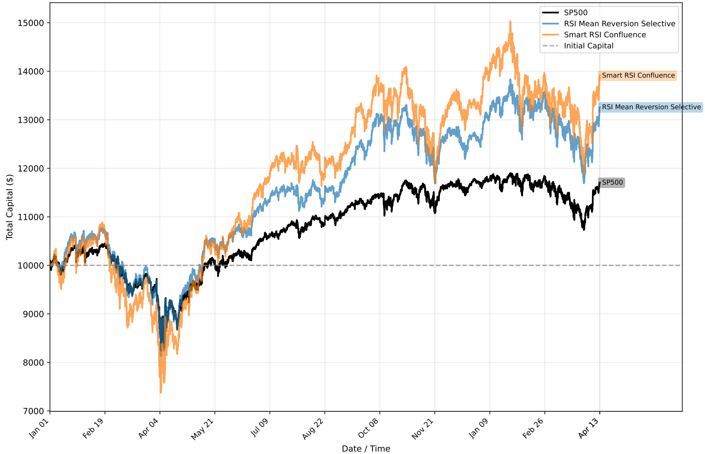
Penguin Capital Curves (25-01-01 to 26-04-13)
