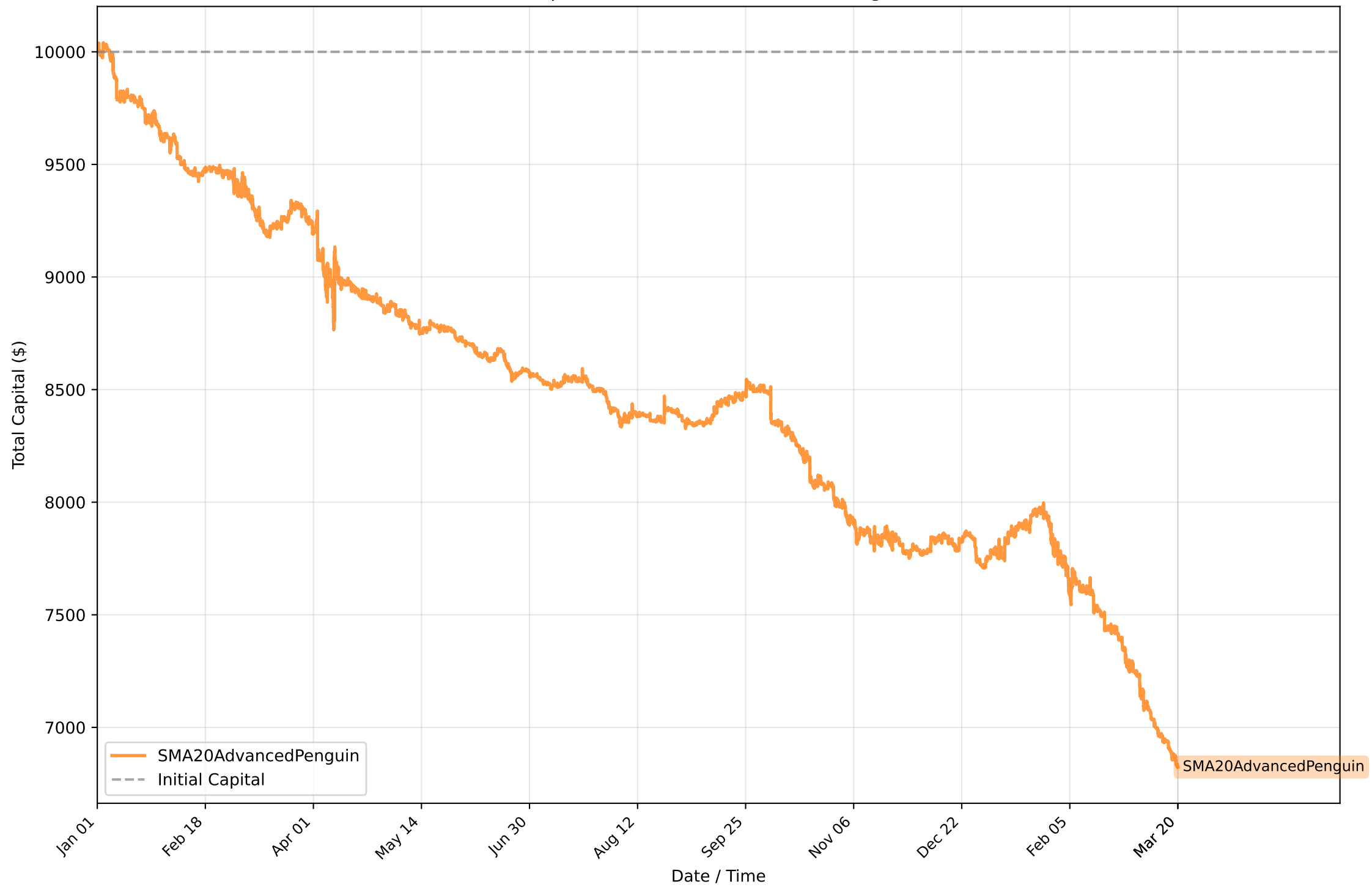
Capital Curve: SMA20AdvancedPenguin
