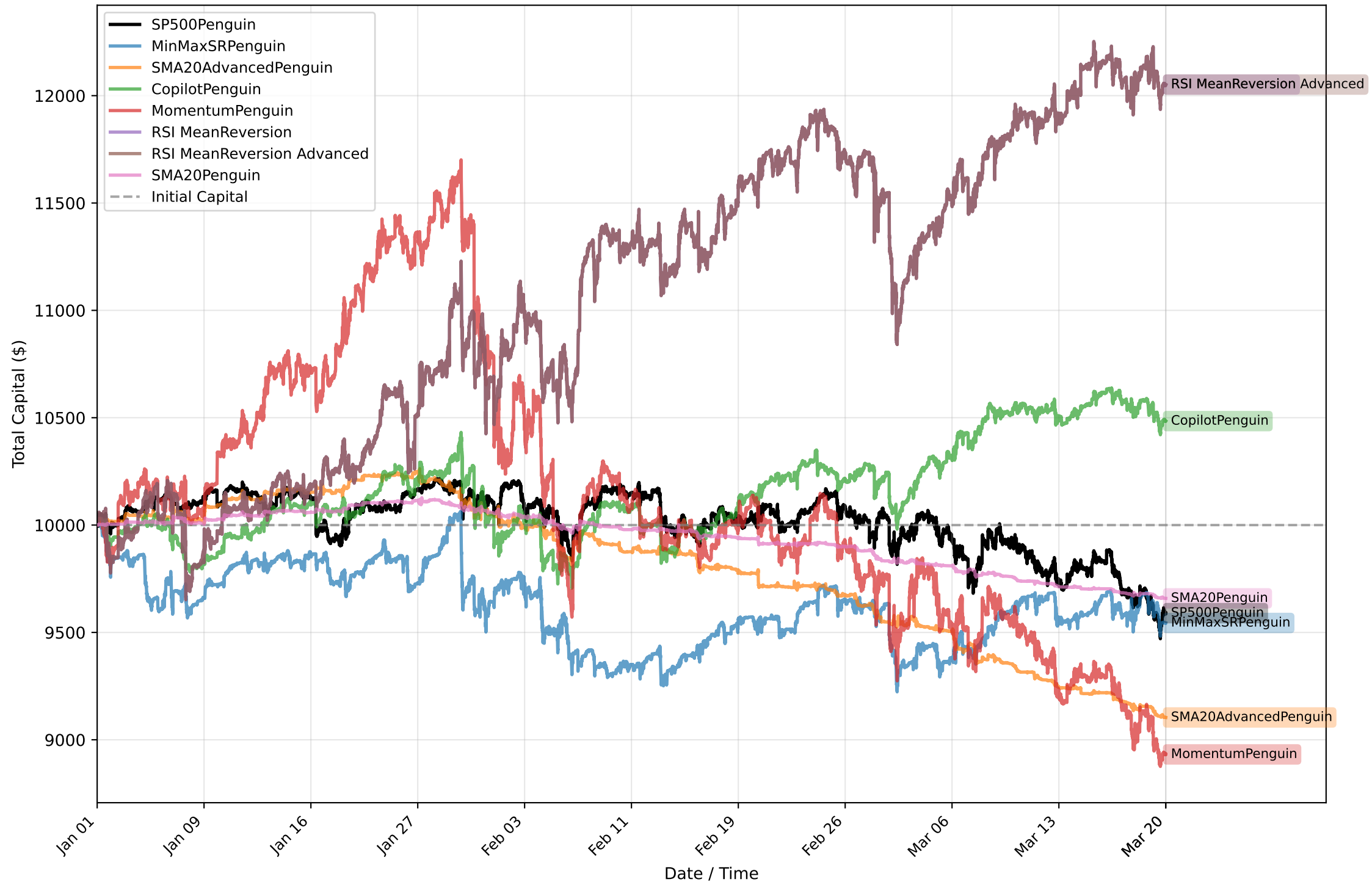
Penguin Capital Curves (26-01-01 to 26-03-20)
