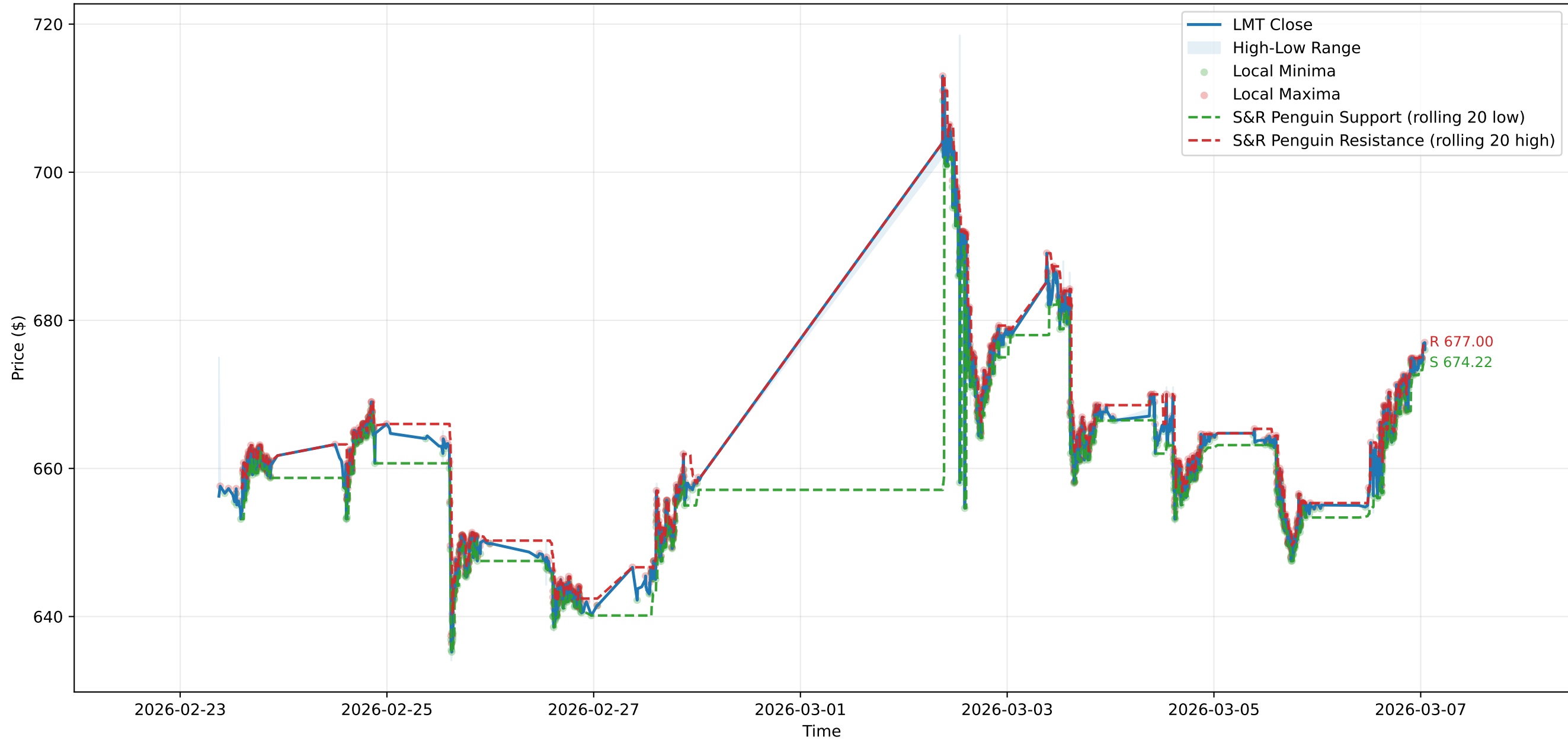
LMT Support & Resistance
