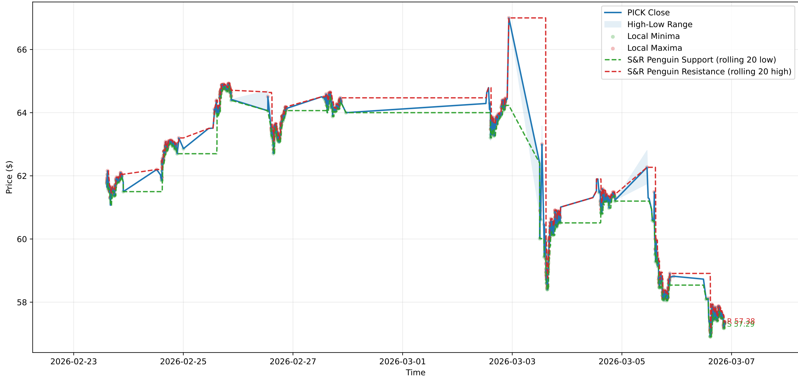
PICK Support & Resistance
