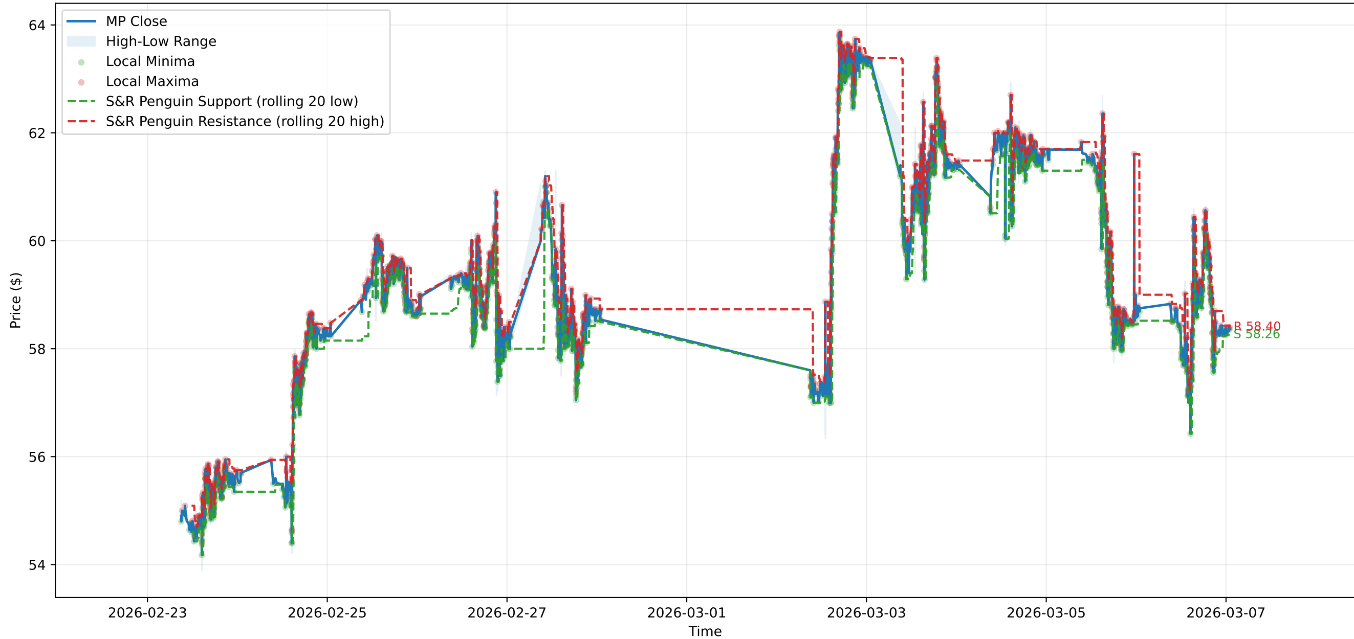
MP Support & Resistance
