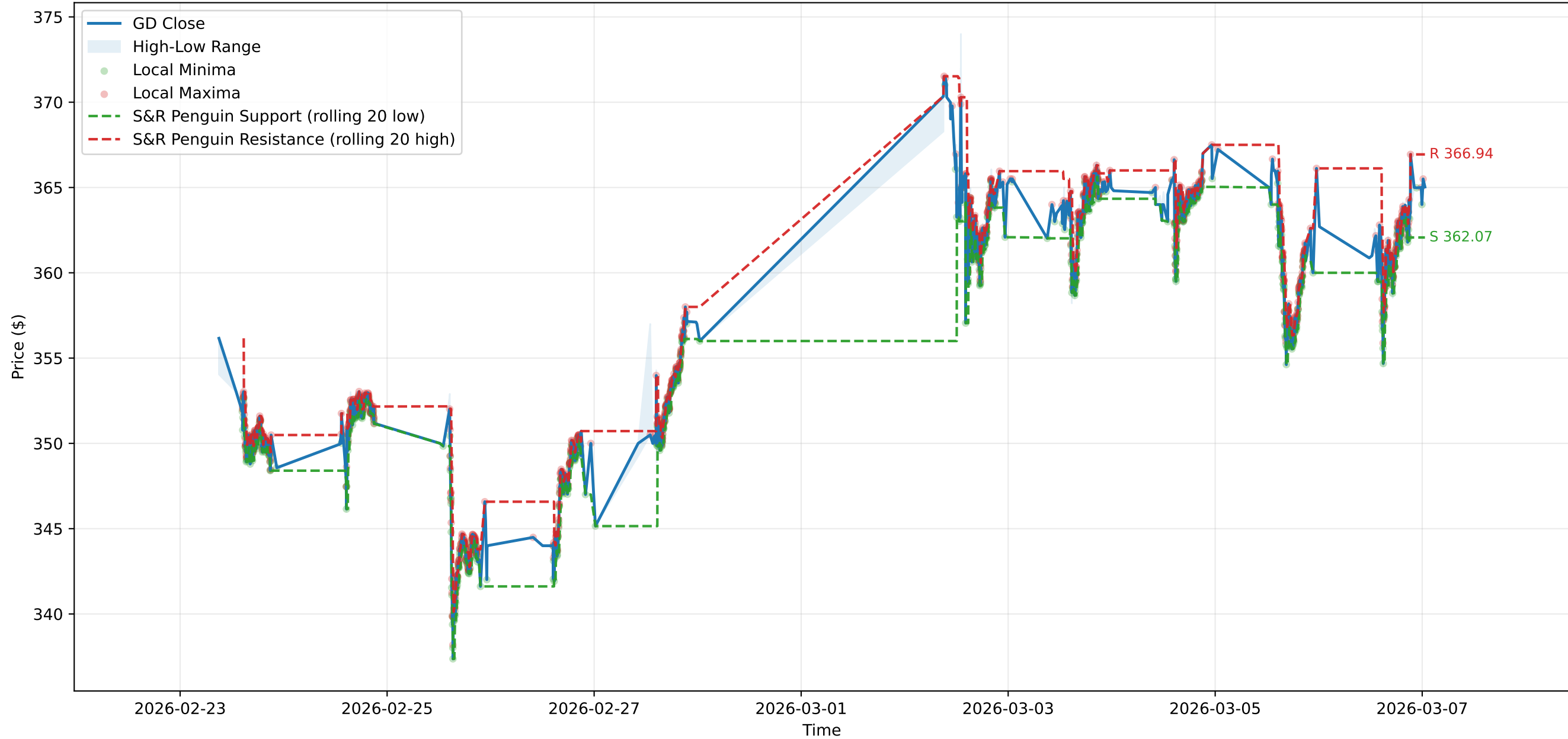
GD Support &amp; Resistance
