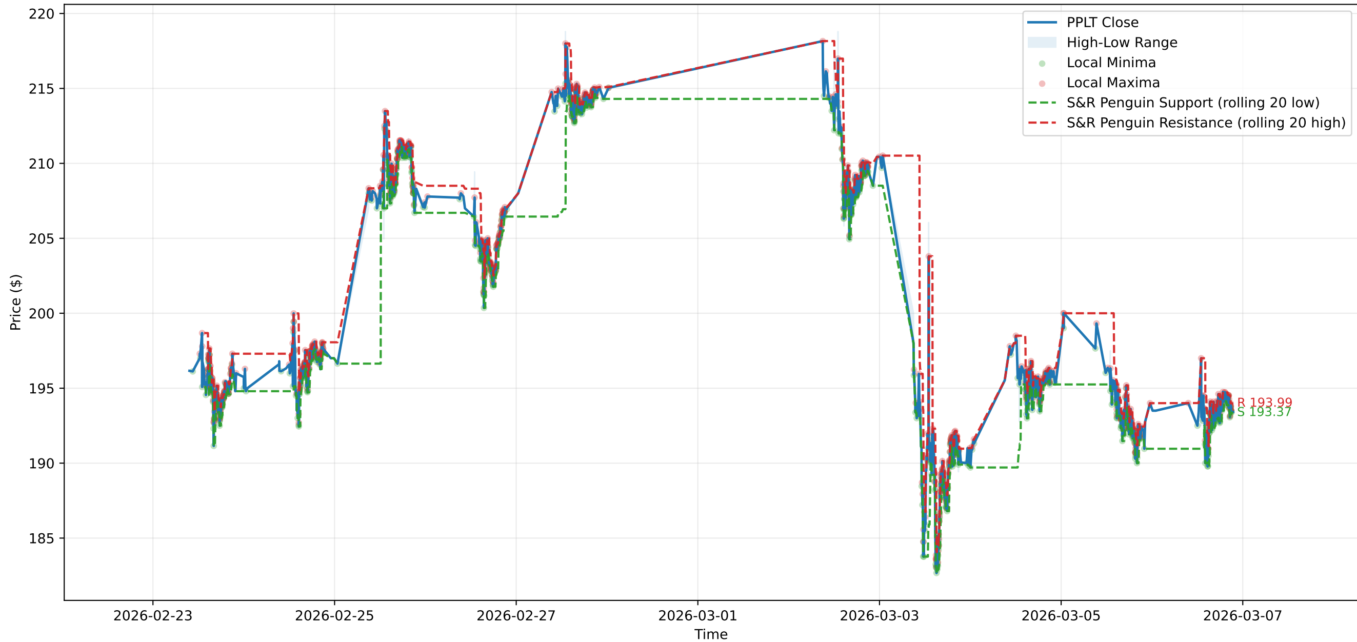
PPLT Support & Resistance
