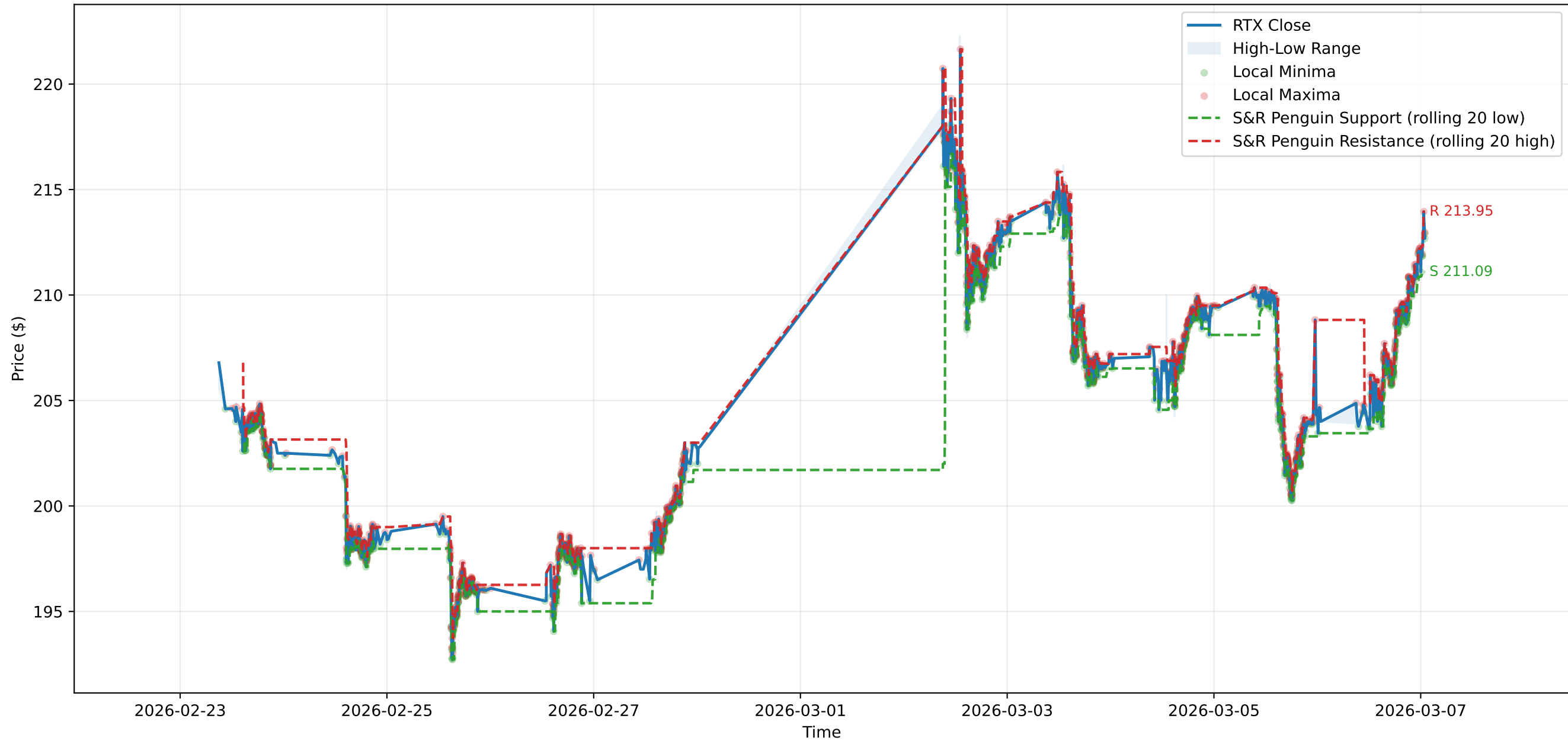
RTX Support & Resistance
