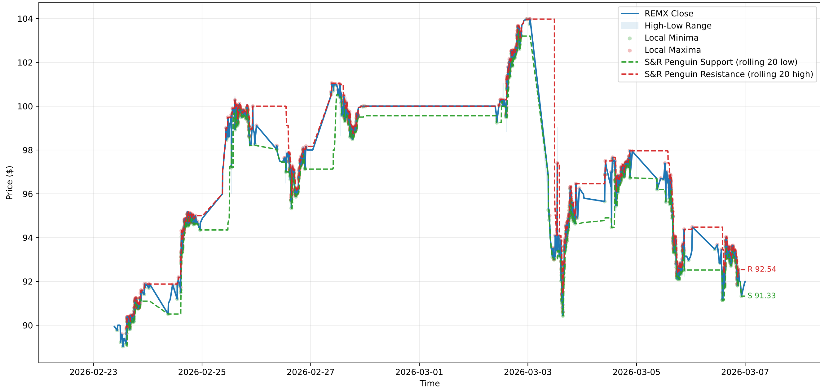
REMX Support & Resistance
