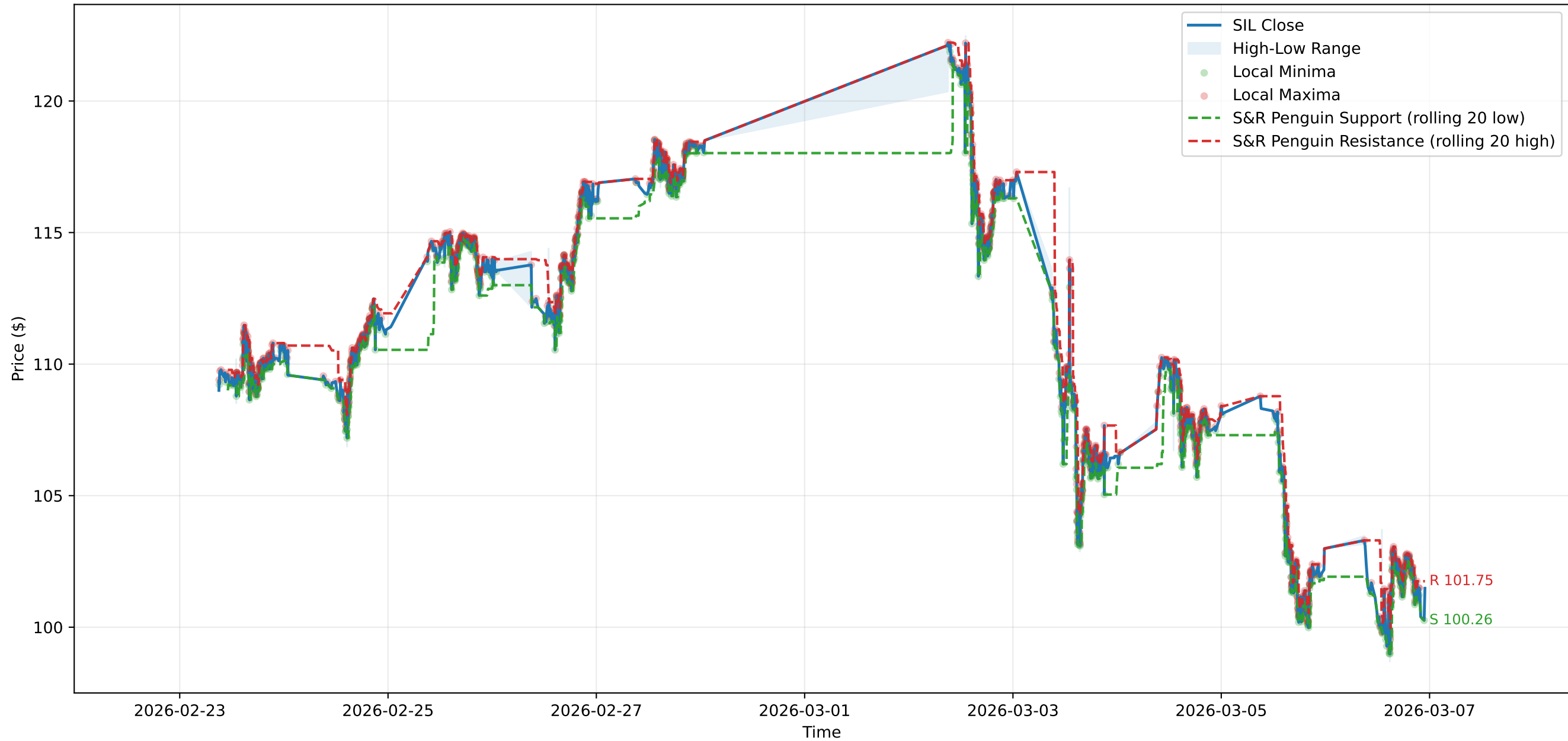
SIL Support & Resistance
