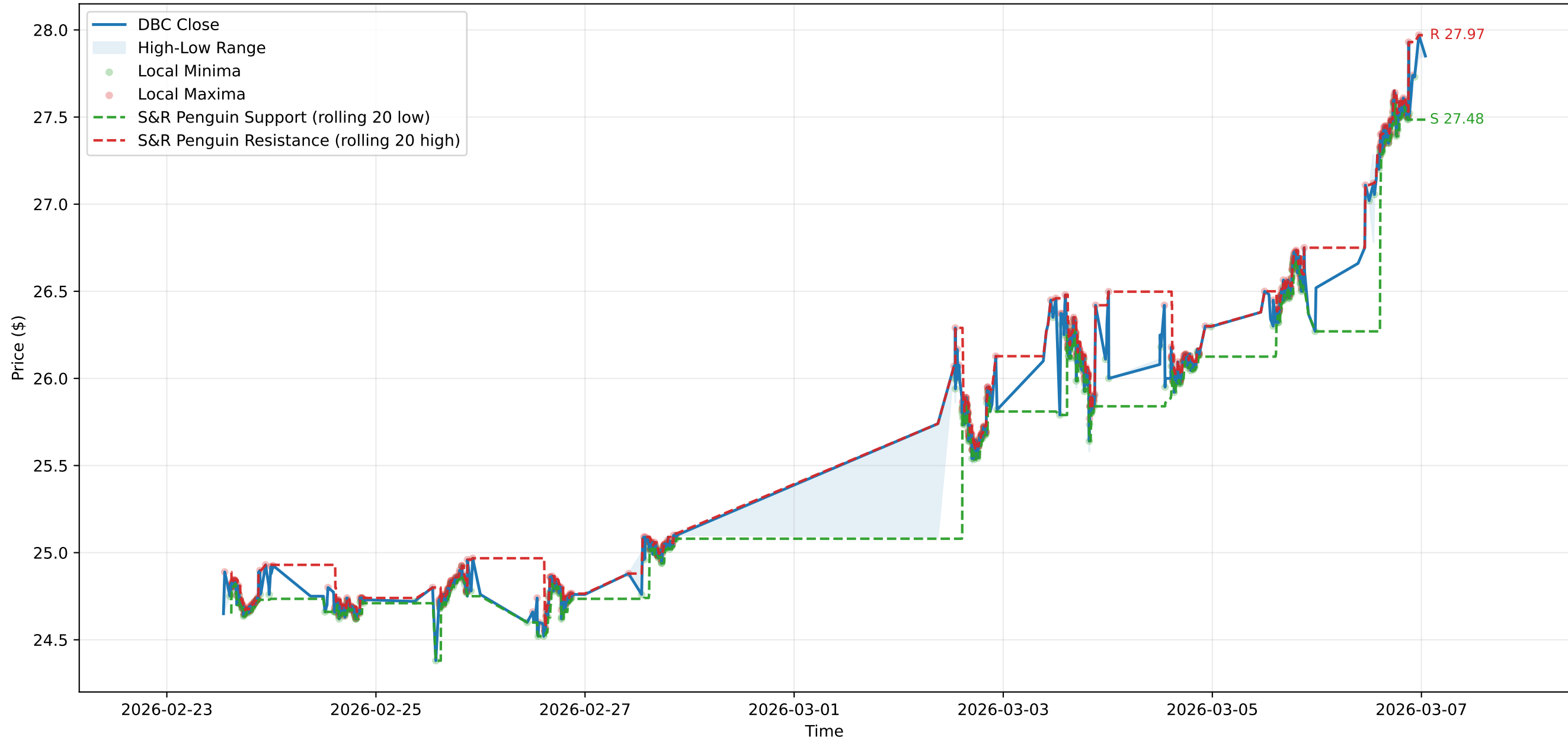
DBC Support & Resistance
