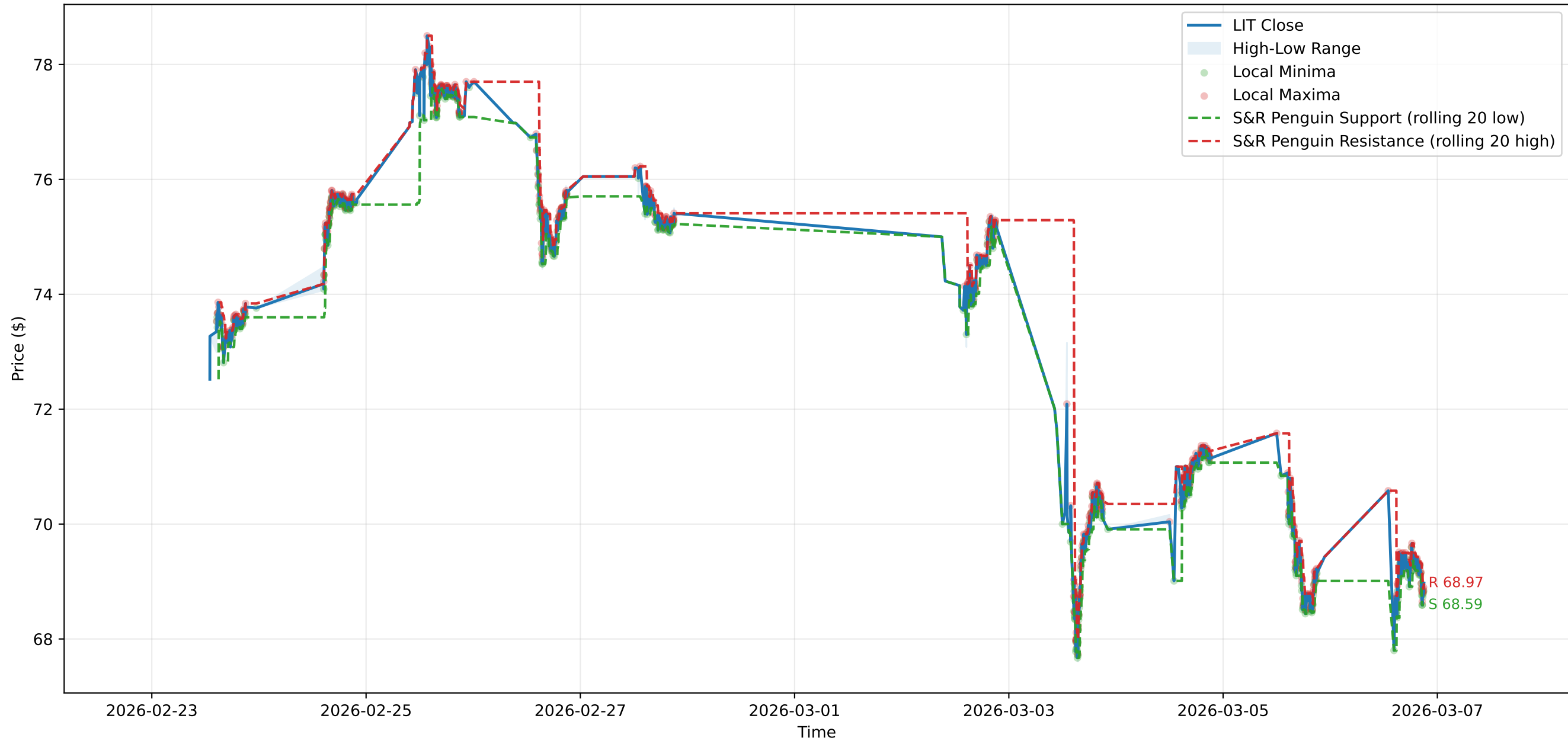
LIT Support &amp; Resistance
