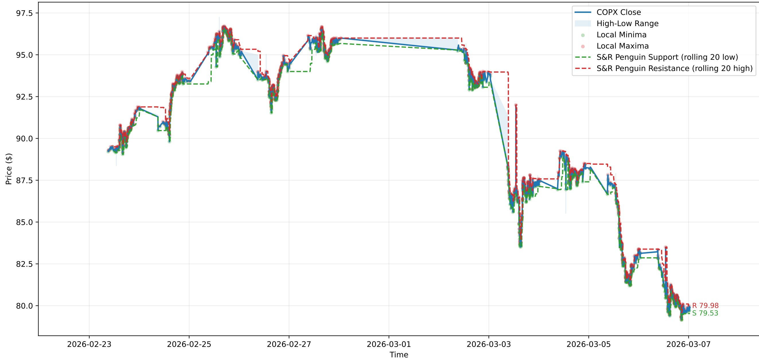
COPX Support &amp; Resistance
