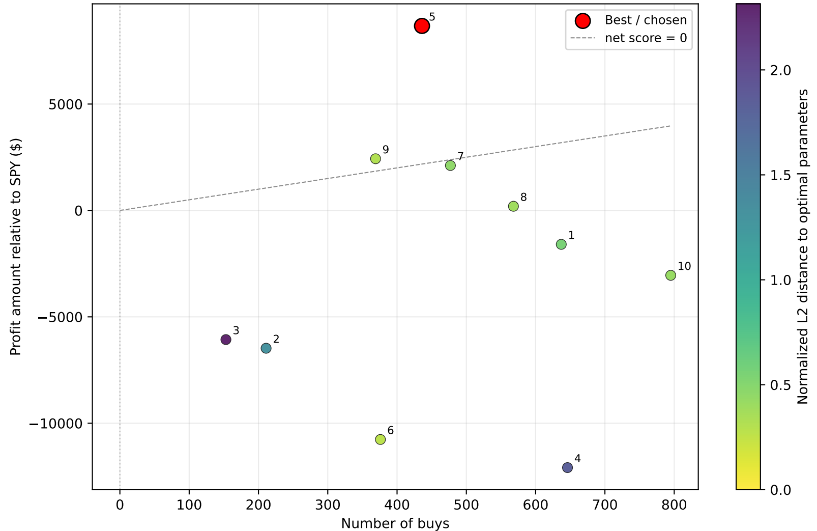
Adv_SELL_TP4 buy-count vs profit relative to SPY
