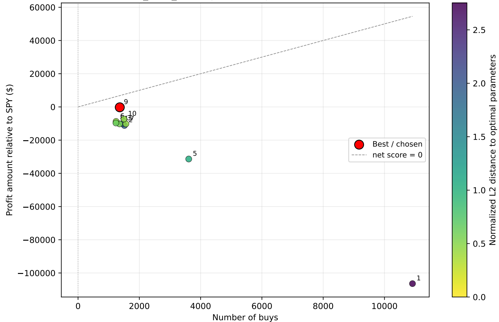
Adv_SELL_TP2 buy-count vs profit relative to SPY
