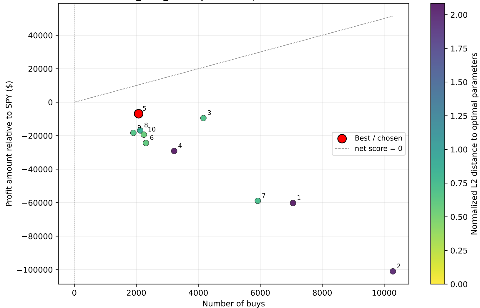
Adv_SELL_TP1 buy-count vs profit relative to SPY
