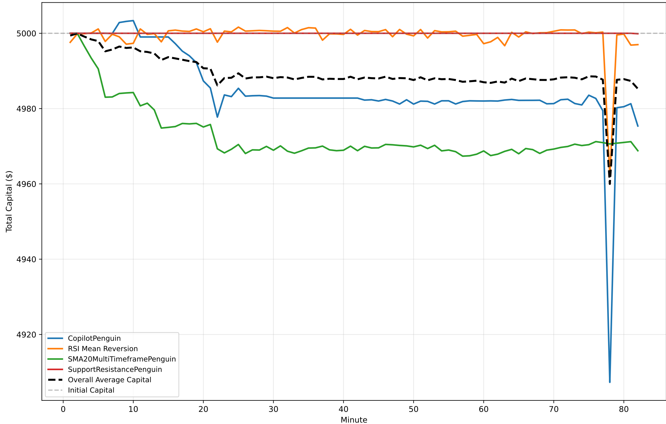
Penguin Capital Curves
