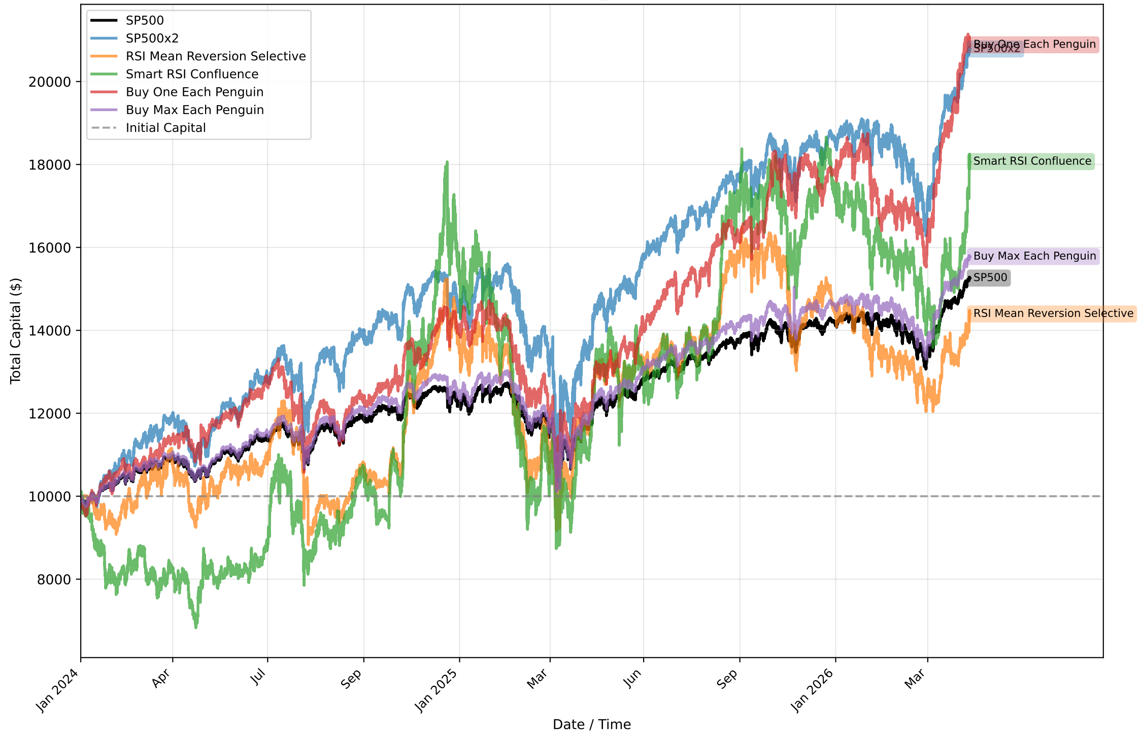
Penguin Capital Curves (LIST_5) (24-01-02 to 26-05-11)
