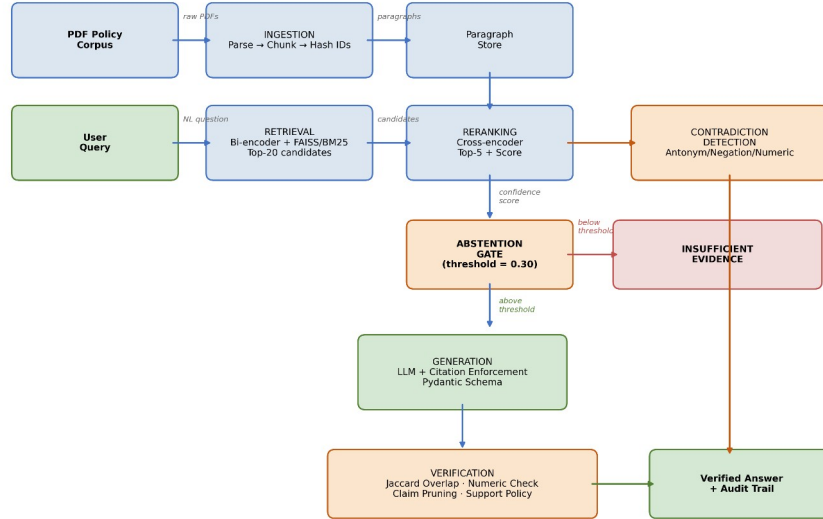
Figure 2.1: End-to-end pipeline from PDF ingestion through retrieval, reranking, abstention, generation, and verification.
