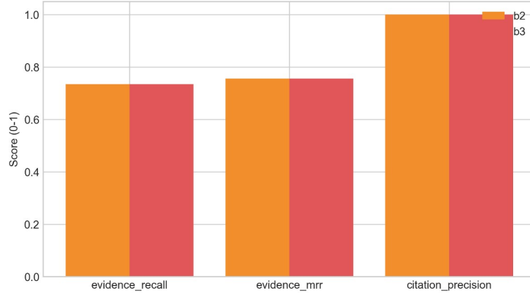
Figure 4.2: Retrieval quality, B2 vs B3 on Recall@5, MRR, and Precision@5.
