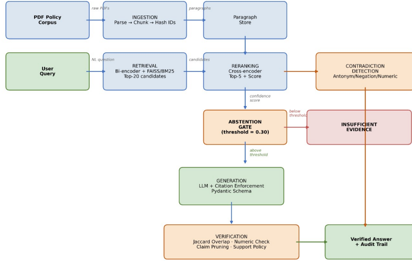
Figure 2.2: End-to-end pipeline from PDF ingestion through retrieval, reranking, abstention, generation, and verification.
