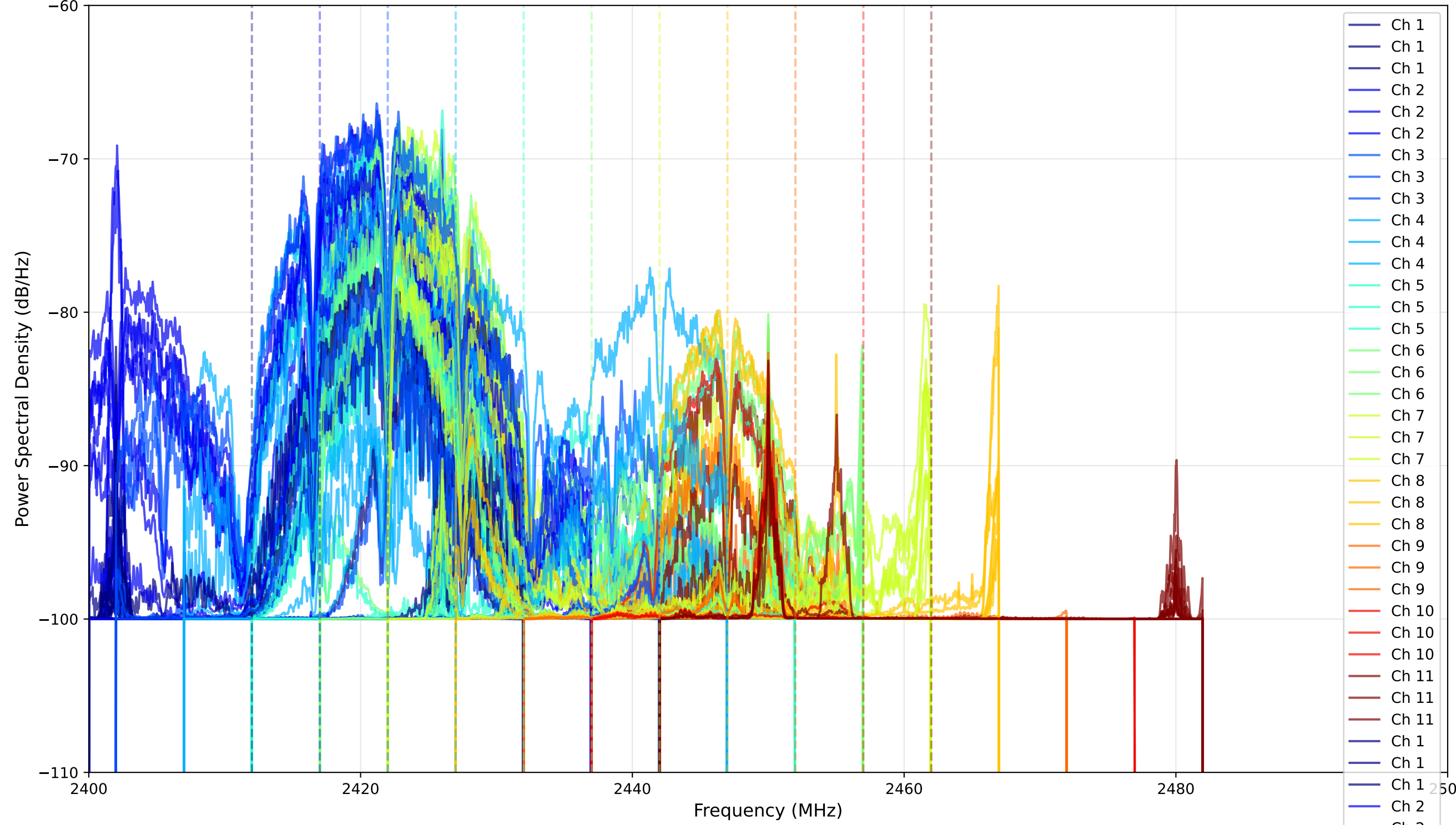
WiFi 2.4GHz Band - No AP Data
