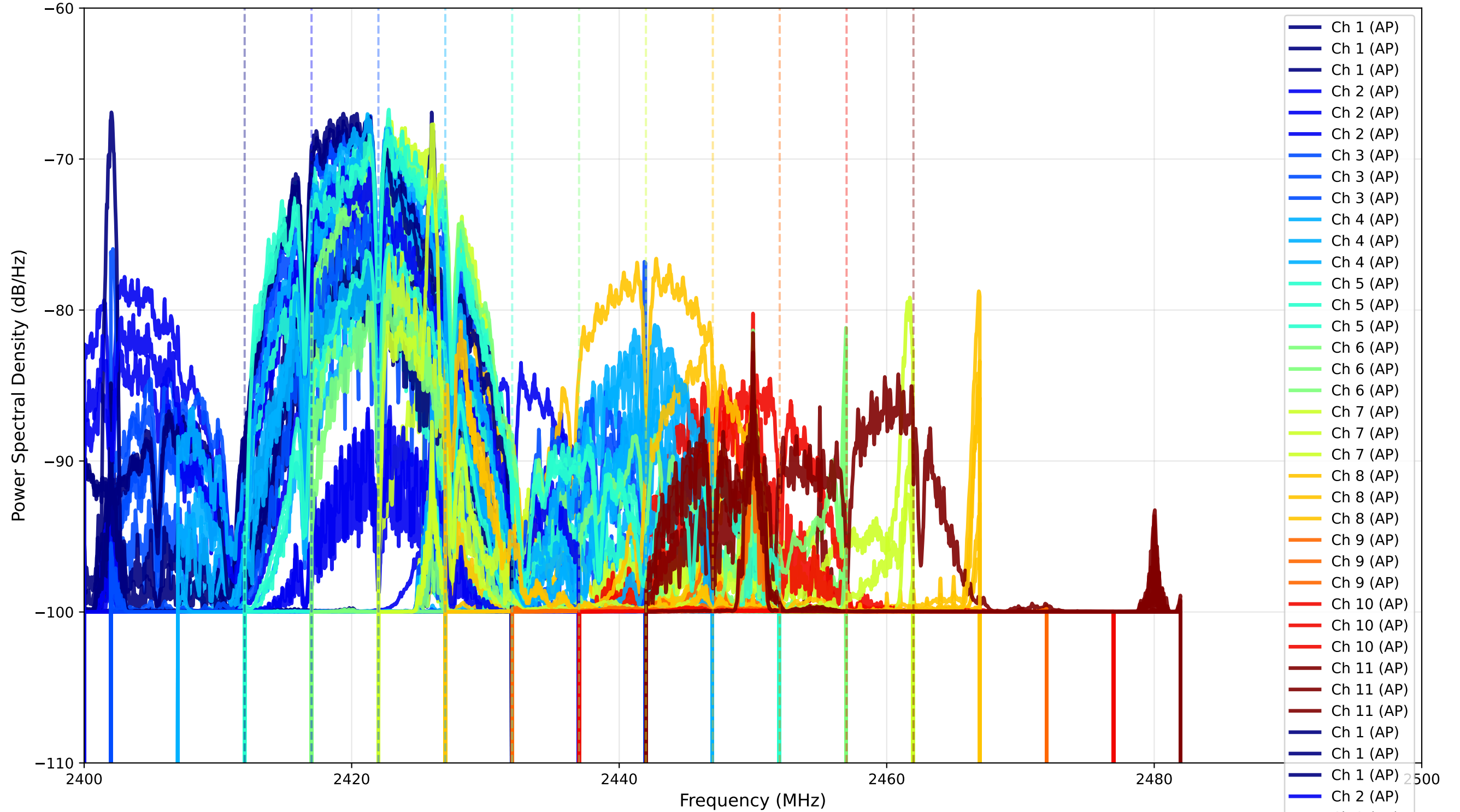
WiFi 2.4GHz Band - All Channels
