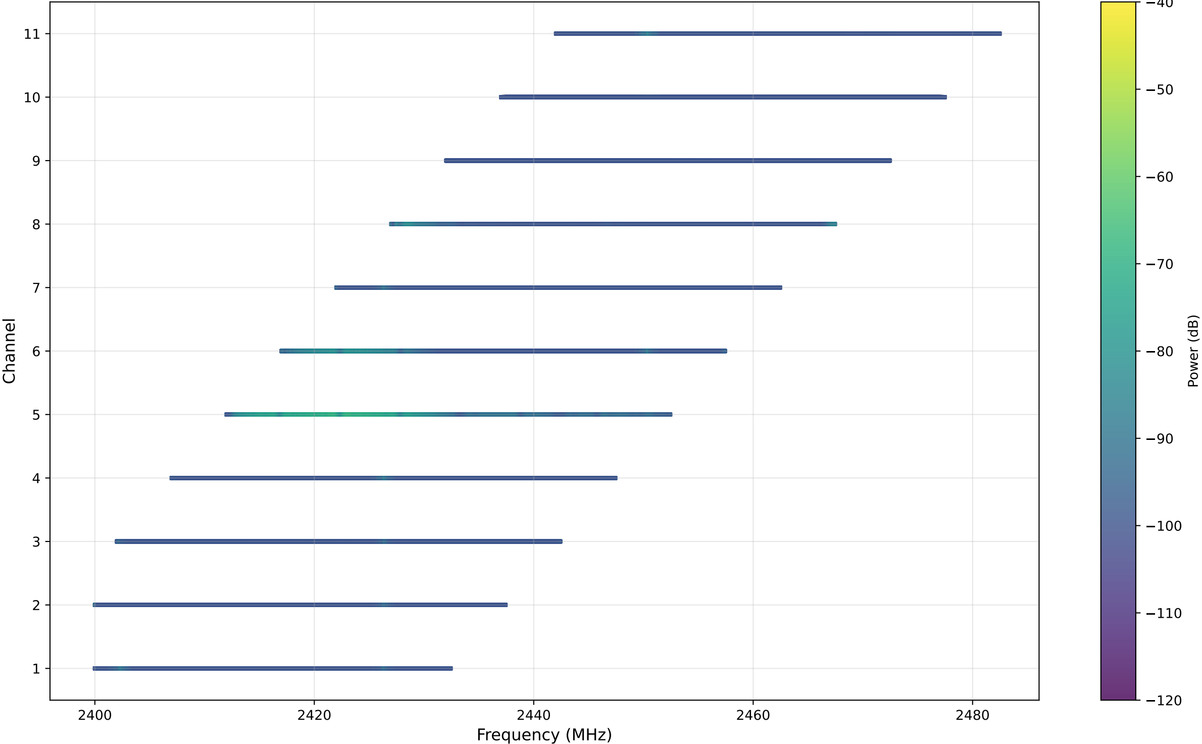
WiFi Channel Spectrum Heatmap
