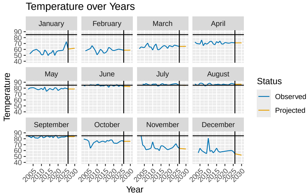
Figure 5.1: This figure shows the mean temperature throughout each year from 2002 to 2025. The line shows the threshold where a power plant would need to run at reduced risk. The projected temperature is denoted by years after the vertical line at the start 2026.
