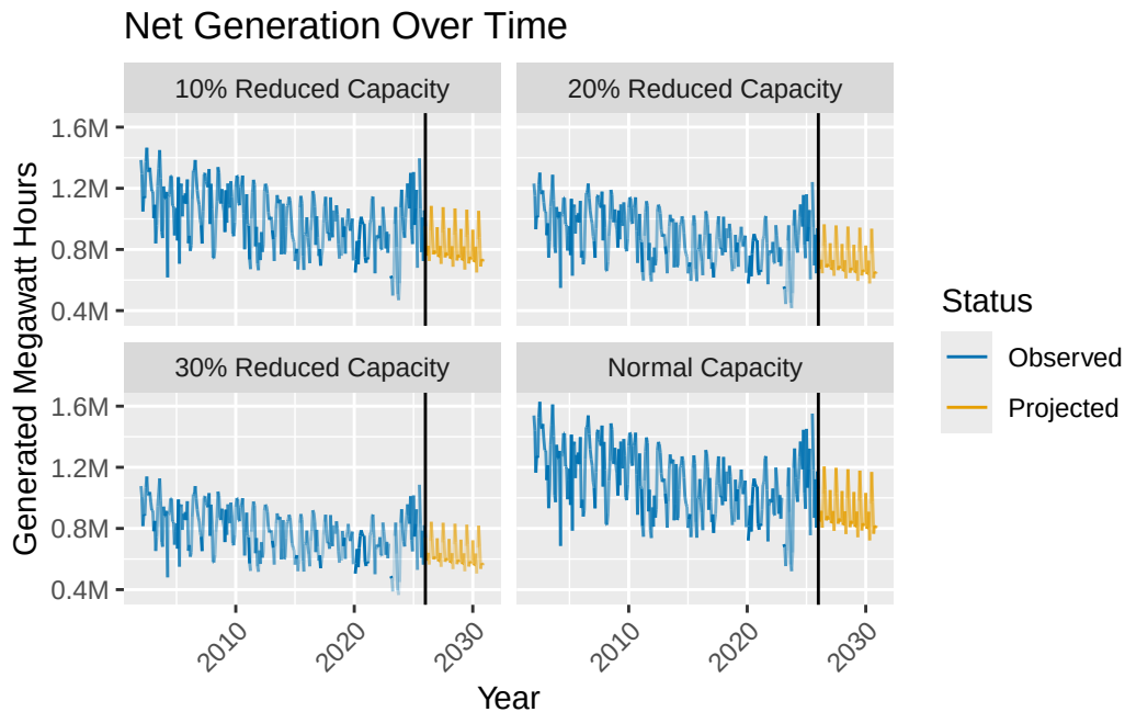
Figure 5.2: This figure shows the generation proficiency at different operational capabilities at a given time. Transparency is denoted by percentage consumed. The projected Net generation is denoted by years after the vertical line at the start 2026.
