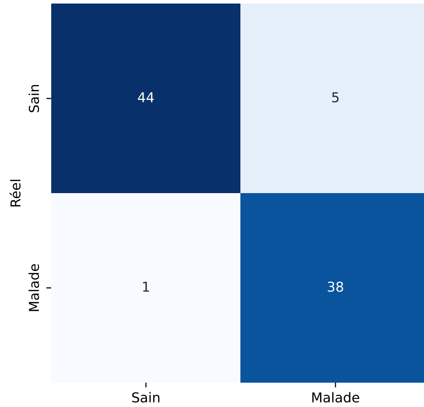
Voting Ensemble Acc: 0.932
