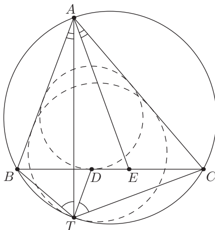
Figure 4.8B. Segments \overline{AT} and \overline{AE} are isogonal in \triangle ABC , while segments \overline{TD} and \overline{TA} are isogonal in \triangle TBC .
