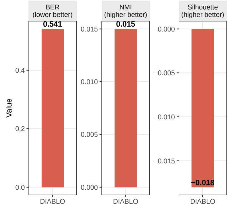
(C) Latent space quality metrics
