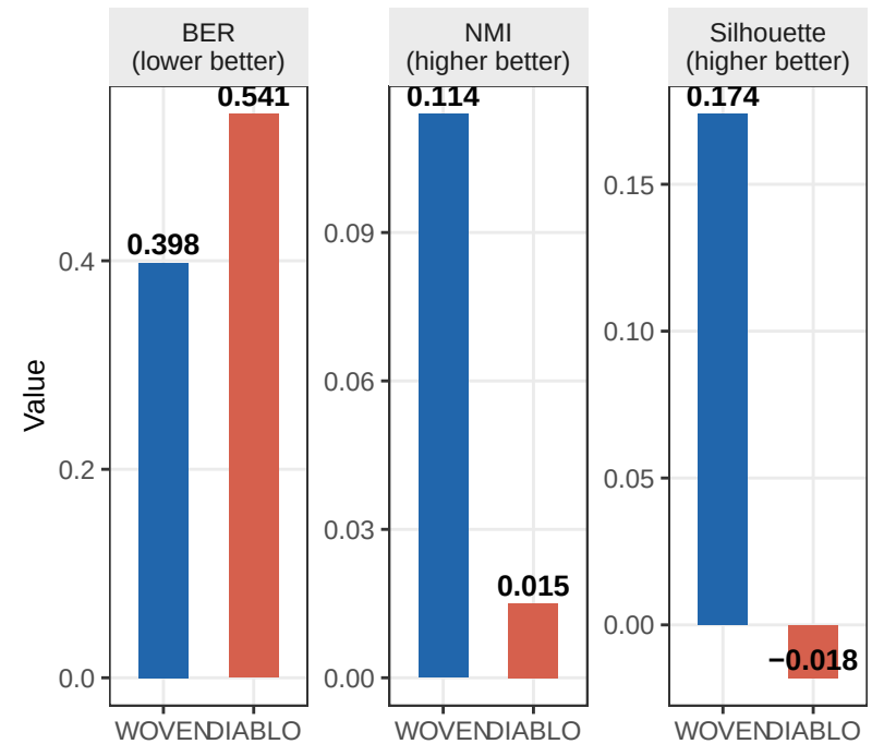
(C) Latent space quality metrics
