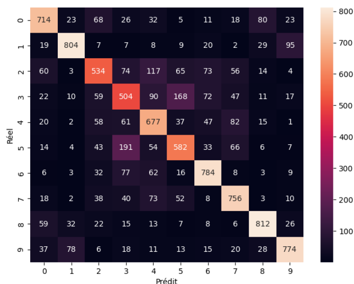
Figure 7 — Matrice de confusion
