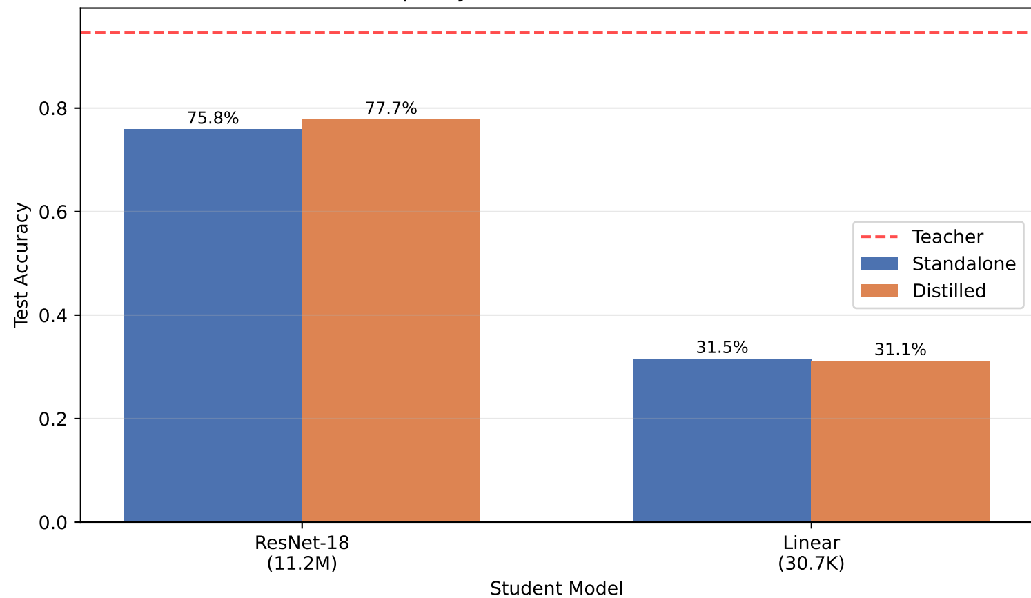
Scenario A: Capacity Mismatch — Standalone vs Distilled
