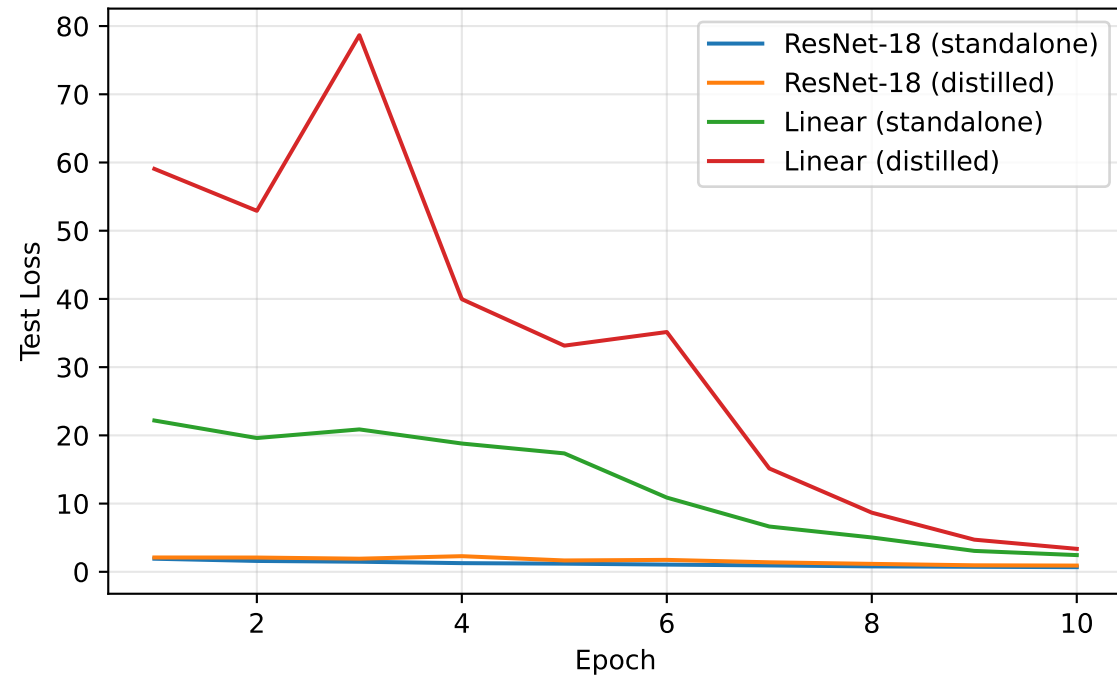
Scenario A — Loss
