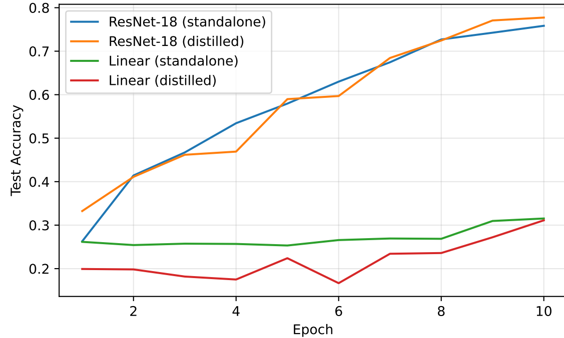
Scenario A — Accuracy
